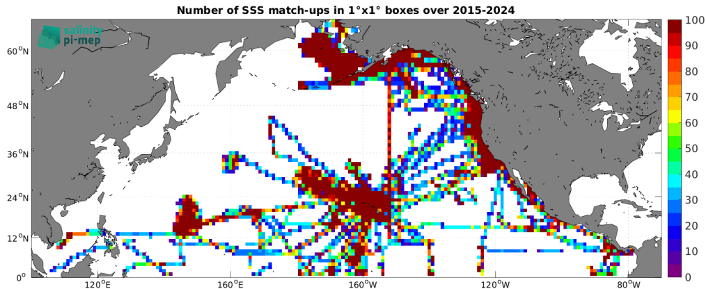
Figure 5: Number of SSS match-ups between TSG (SAMOS) SSS and the SMAP SSS L3 v5.0 - 8-Day running (JPL) SSS product for the North Pacific Ocean Pi-MEP region over 1^\circ \times 1^\circ boxes and for the full satellite product period.
