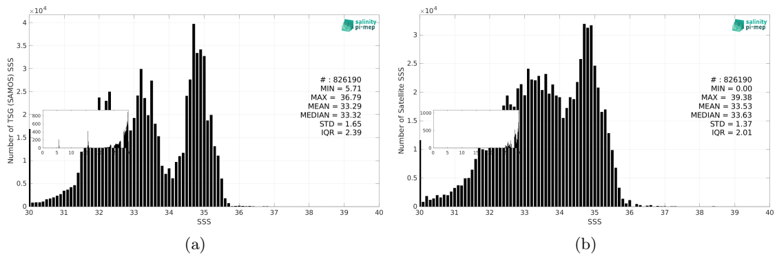
Figure 3: Histograms of SSS from TSG (SAMOS) (a) and SMAP SSS L3 v5.0 - 8-Day running (JPL) (b) considering all match-up pairs per bins of 0.1 over the North Pacific Ocean Pi-MEP region and for the full satellite product period.
