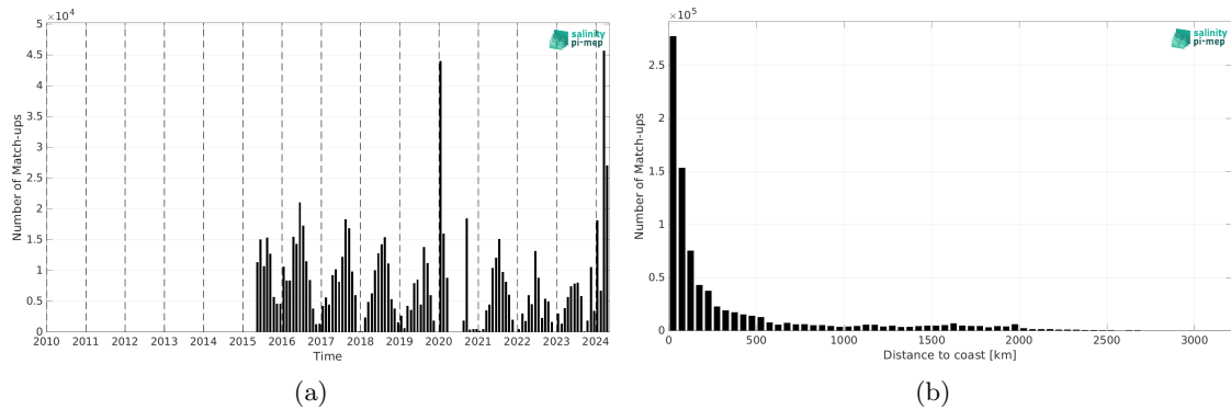
Figure 2: Number of match-ups between TSG (SAMOS) and SMAP SSS L3 v5.0 - 8-Day running (JPL) SSS as a function of time (a) and as function of the distance to coast (b) over the North Pacific Ocean Pi-MEP region and for the full satellite product period.
