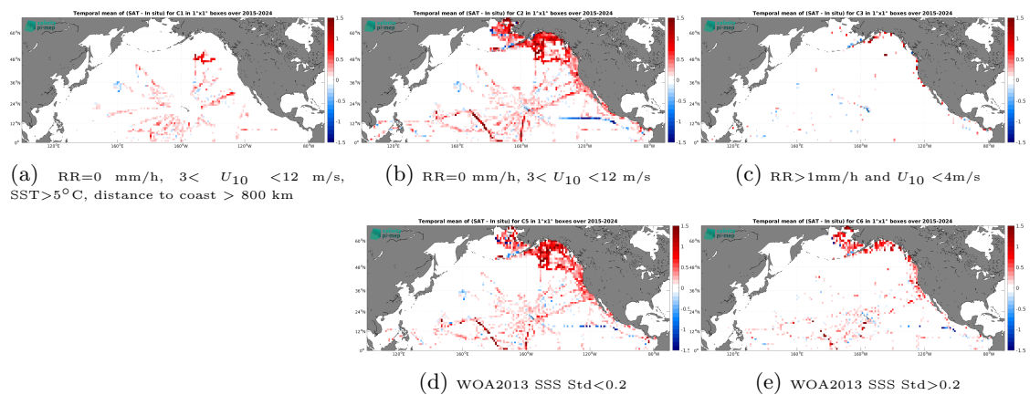
Figure 14: Temporal mean gridded over spatial boxes of size 1^\circ \times 1^\circ of \Delta\text{SSS} (SMAP SSS L3 v5.0 - 8-Day running (JPL) - TSG (SAMOS)) for 5 different subdatasets corresponding to: RR=0 mm/h, 3 < U_{10} < 12 m/s, SST > 5°C, distance to coast > 800 km (a), RR=0 mm/h, 3 < U_{10} < 12 m/s (b), RR > 1mm/h and U_{10} < 4 m/s (c), WOA2013 SSS Std < 0.2 (d), WOA2013 SSS Std > 0.2 (e).
