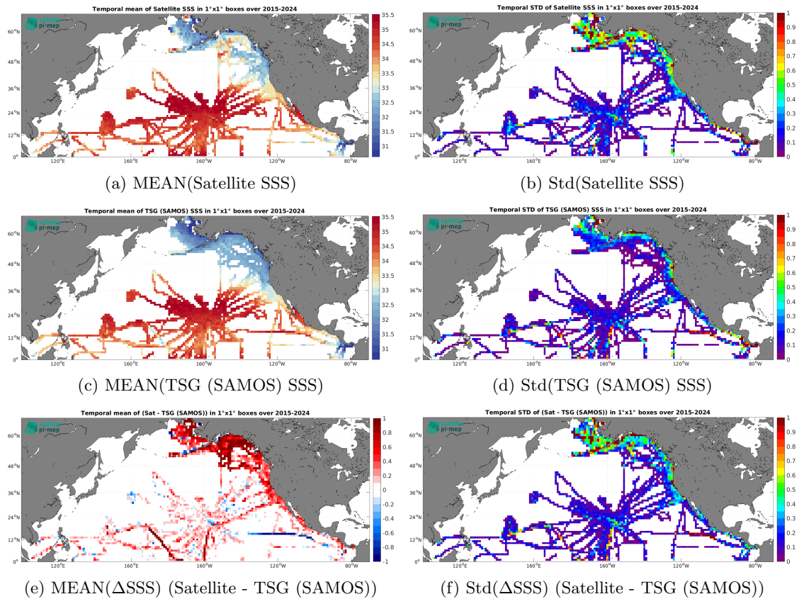
Figure 7: Temporal mean (left) and Std (right) of SSS from SMAP SSS L3 v5.0 - 8-Day running (JPL) (top), TSG (SAMOS) (middle), and of \Delta SSS (Satellite - TSG (SAMOS)). Only match-up pairs are used to generate these maps.
