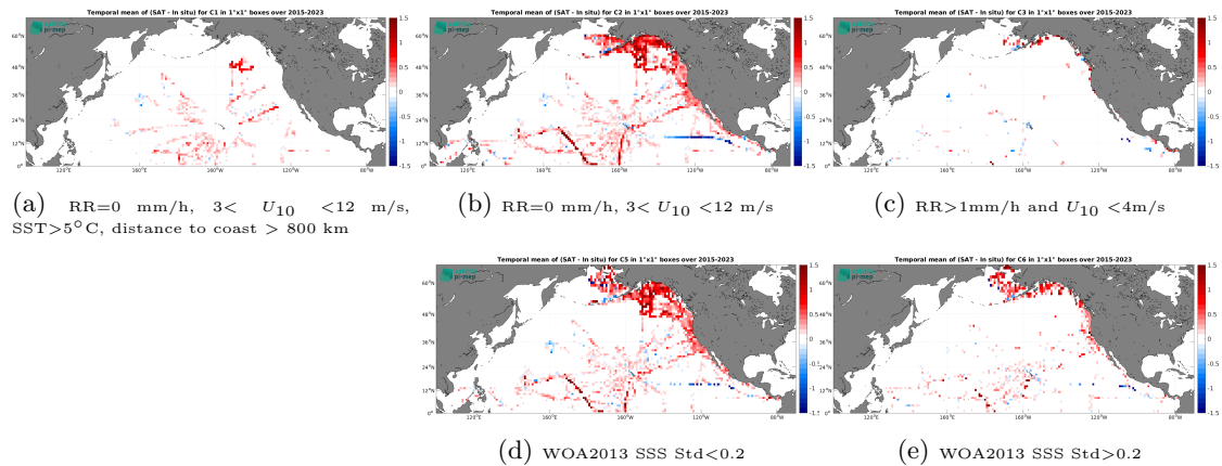
Figure 12: Temporal mean gridded over spatial boxes of size 1^\circ \times 1^\circ of \Delta\text{SSS} (SMAP SSS L3 v5.0 - 8-Day running (JPL) - TSG (SAMOS)) for 5 different subdatasets corresponding to:RR=0 mm/h, 3 < U_{10} < 12 m/s, SST >5^\circ\text{C} , distance to coast > 800 km (a), RR=0 mm/h, 3 < U_{10} < 12 m/s (b), RR >1 mm/h and U_{10} < 4 m/s (c), WOA2013 SSS Std <0.2 (d), WOA2013 SSS Std >0.2 (e).
