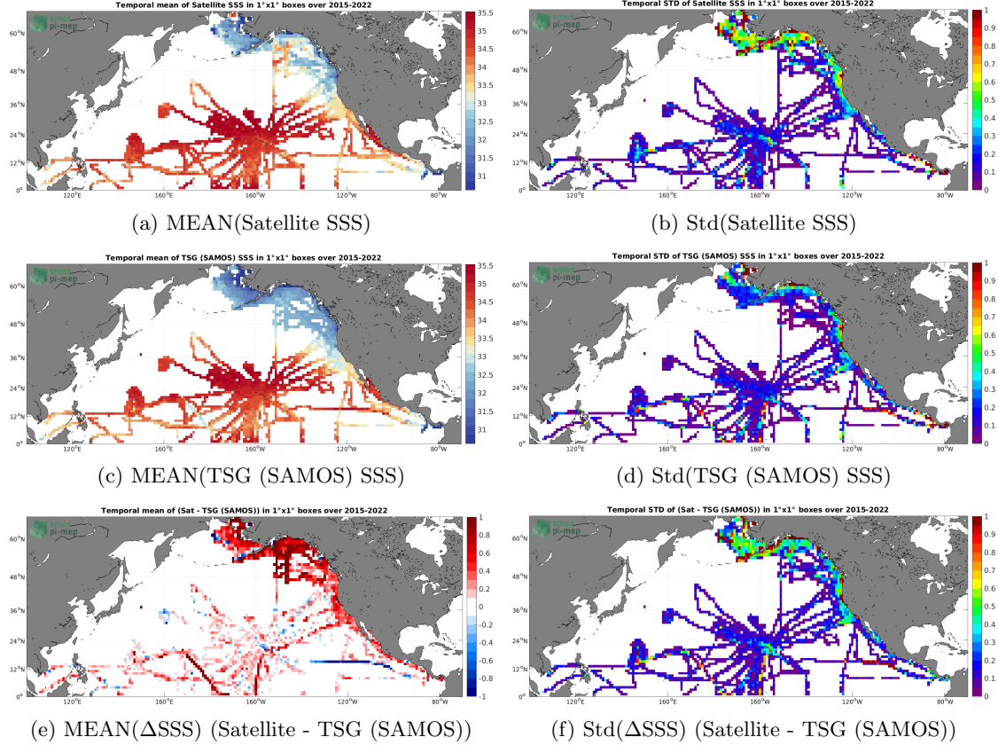
Figure 6: Temporal mean (left) and Std (right) of SSS from SMAP SSS L3 v5.0 - 8-Day running (JPL) (top), TSG (SAMOS) (middle), and of \Delta\text{SSS} (Satellite - TSG (SAMOS)). Only match-up pairs are used to generate these maps.
