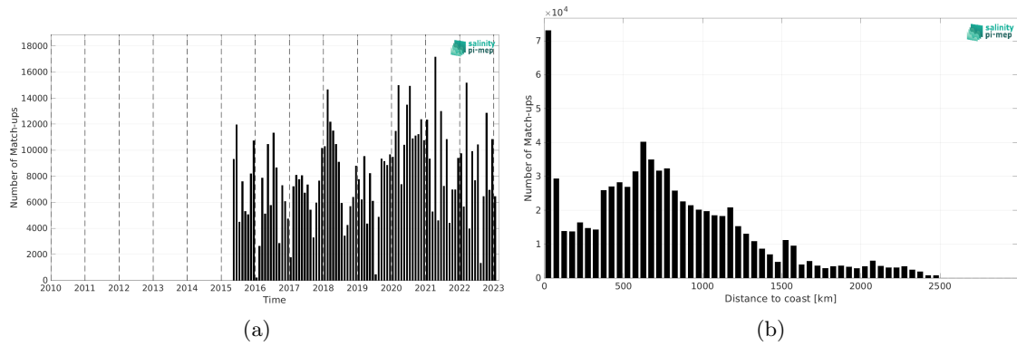
Figure 2: Number of match-ups between TSG (LEGOS-DM) and SMAP SSS L3 v5.0 - 8-Day running (JPL) SSS as a function of time (a) and as function of the distance to coast (b) over the North Pacific Ocean Pi-MEP region and for the full satellite product period.
