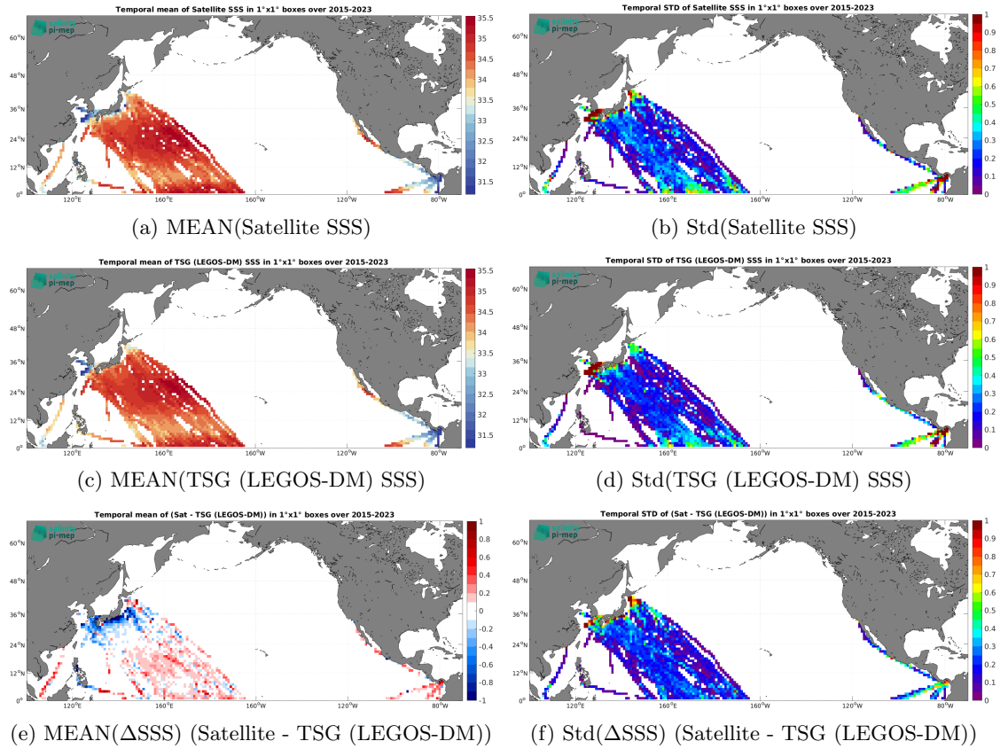
Figure 7: Temporal mean (left) and Std (right) of SSS from SMAP SSS L3 v5.0 - 8-Day running (JPL) (top), TSG (LEGOS-DM) (middle), and of \Delta SSS (Satellite - TSG (LEGOS-DM)). Only match-up pairs are used to generate these maps.
