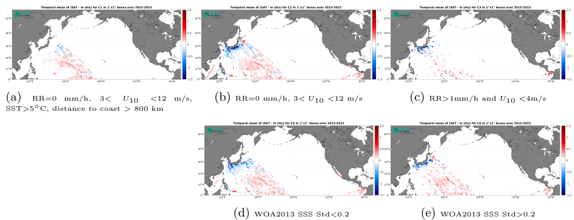
Figure 14: Temporal mean gridded over spatial boxes of size 1^\circ \times 1^\circ of \Delta\text{SSS} (SMAP SSS L3 v5.0 - 8-Day running (JPL) - TSG (LEGOS-DM)) for 5 different subdatasets corresponding to:RR=0 mm/h, 3 < U_{10} < 12 m/s, SST>5°C, distance to coast > 800 km (a), RR=0 mm/h, 3 < U_{10} < 12 m/s (b), RR>1mm/h and U_{10} < 4 m/s (c), WOA2013 SSS Std<0.2 (d), WOA2013 SSS Std>0.2 (e).
