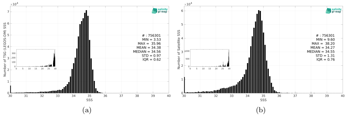
Figure 3: Histograms of SSS from TSG (LEGOS-DM) (a) and SMAP SSS L3 v5.0 - 8-Day running (JPL) (b) considering all match-up pairs per bins of 0.1 over the North Pacific Ocean Pi-MEP region and for the full satellite product period.
