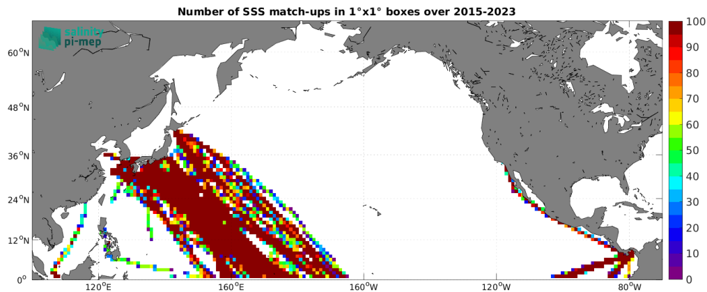
Figure 5: Number of SSS match-ups between TSG (LEGOS-DM) SSS and the SMAP SSS L3 v5.0 - 8-Day running (JPL) SSS product for the North Pacific Ocean Pi-MEP region over 1^\circ \times 1^\circ boxes and for the full satellite product period.
