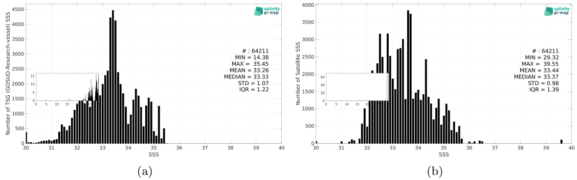
Figure 3: Histograms of SSS from TSG (GOSUD-Research-vessel) (a) and SMAP SSS L3 v5.0 - 8-Day running (JPL) (b) considering all match-up pairs per bins of 0.1 over the North Pacific Ocean Pi-MEP region and for the full satellite product period.
