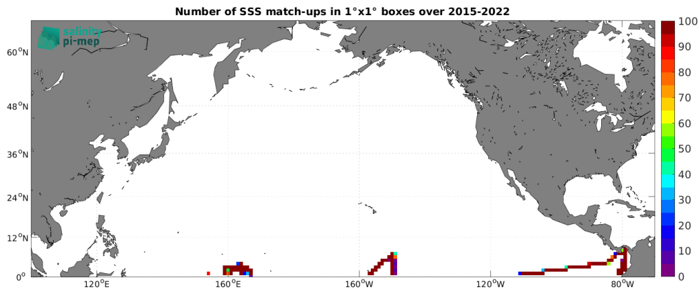
Figure 5: Number of SSS match-ups between TSG (GOSUD-Research-vessel) SSS and the SMAP SSS L3 v5.0 - 8-Day running (JPL) SSS product for the North Pacific Ocean Pi-MEP region over 1^\circ \times 1^\circ boxes and for the full satellite product period.
