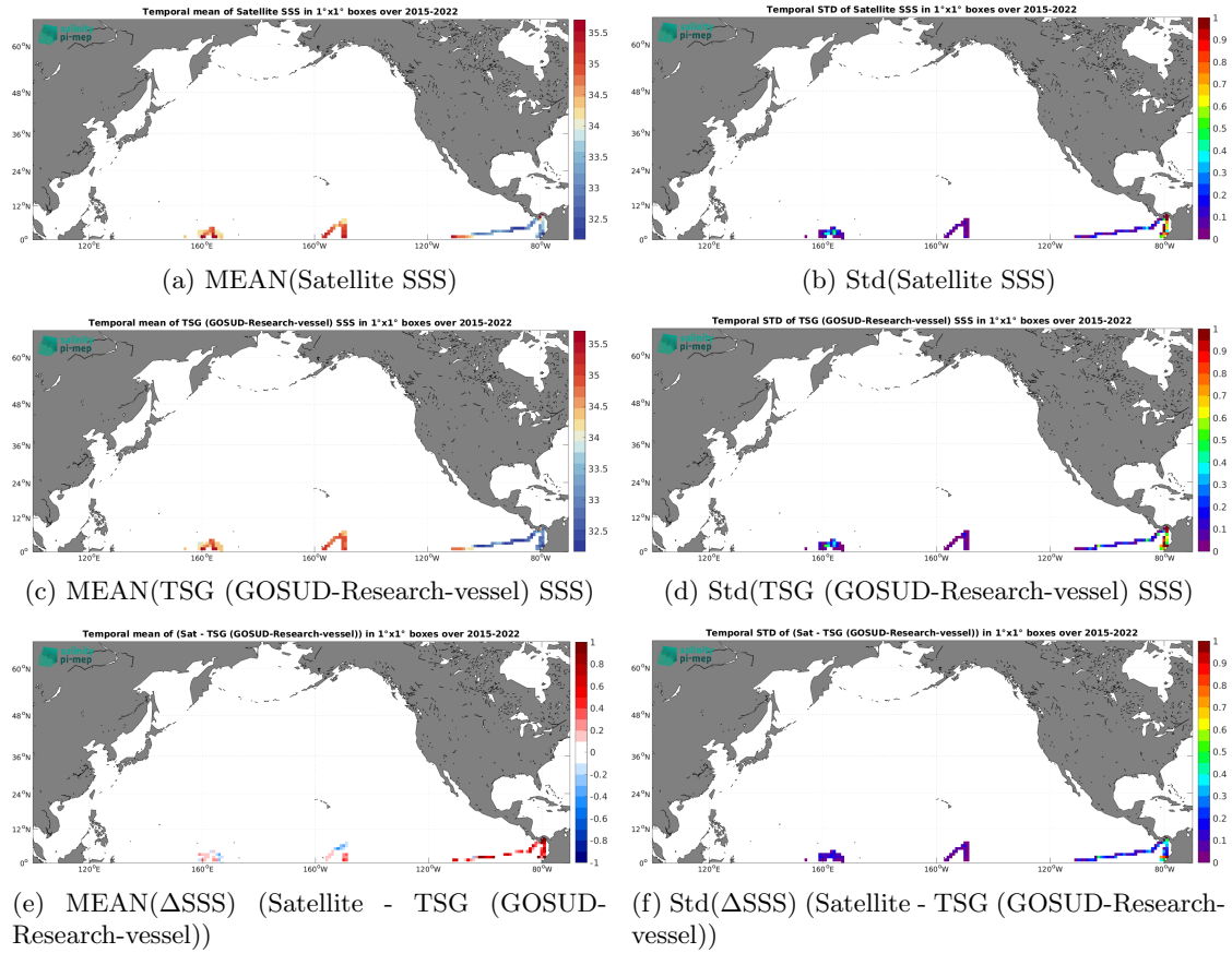
Figure 7: Temporal mean (left) and Std (right) of SSS from SMAP SSS L3 v5.0 - 8-Day running (JPL) (top), TSG (GOSUD-Research-vessel) (middle), and of \Delta SSS (Satellite - TSG (GOSUD-Research-vessel)). Only match-up pairs are used to generate these maps.
