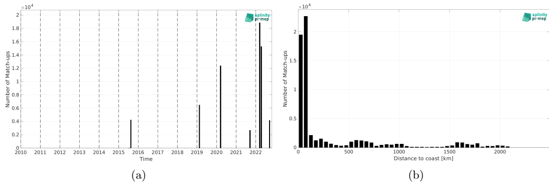
Figure 2: Number of match-ups between TSG (GOSUD-Research-vessel) and SMAP SSS L3 v5.0 - 8-Day running (JPL) SSS as a function of time (a) and as function of the distance to coast (b) over the North Pacific Ocean Pi-MEP region and for the full satellite product period.
