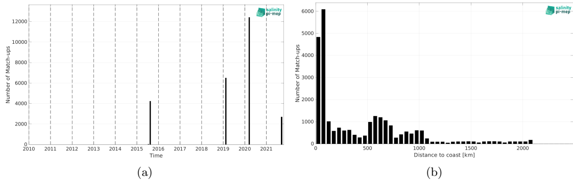
Figure 2: Number of match-ups between TSG (GOSUD-Research-vessel) and SMAP SSS L3 v5.0 - 8-Day running (JPL) SSS as a function of time (a) and as function of the distance to coast (b) over the North Pacific Ocean Pi-MEP region and for the full satellite product period.
