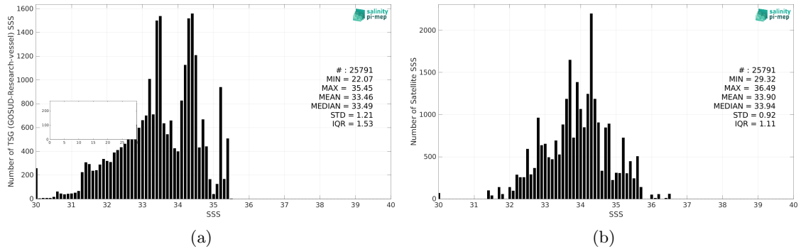
Figure 2: Histograms of SSS from TSG (GOSUD-Research-vessel) (a) and SMAP SSS L3 v5.0 - 8-Day running (JPL) (b) considering all match-up pairs per bins of 0.1 over the North Pacific Ocean Pi-MEP region and for the full satellite product period.
