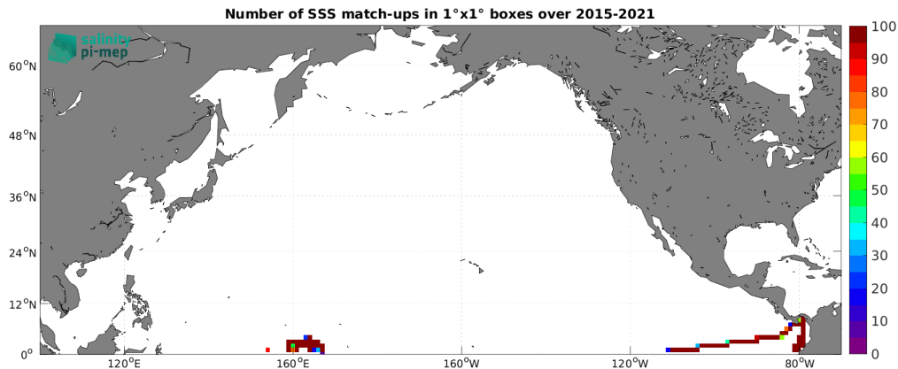
Figure 4: Number of SSS match-ups between TSG (GOSUD-Research-vessel) SSS and the SMAP SSS L3 v5.0 - 8-Day running (JPL) SSS product for the North Pacific Ocean Pi-MEP region over 1^\circ \times 1^\circ boxes and for the full satellite product period.
