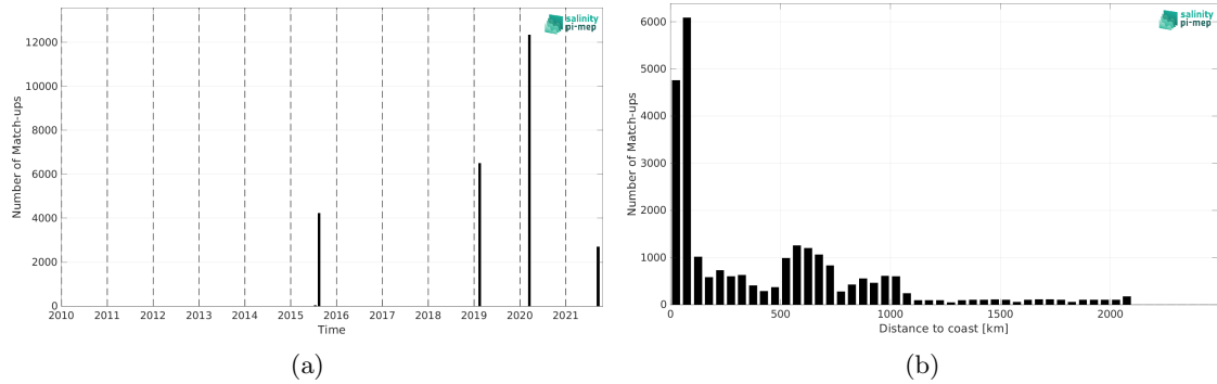
Figure 1: Number of match-ups between TSG (GOSUD-Research-vessel) and SMAP SSS L3 v5.0 - 8-Day running (JPL) SSS as a function of time (a) and as function of the distance to coast (b) over the North Pacific Ocean Pi-MEP region and for the full satellite product period.
