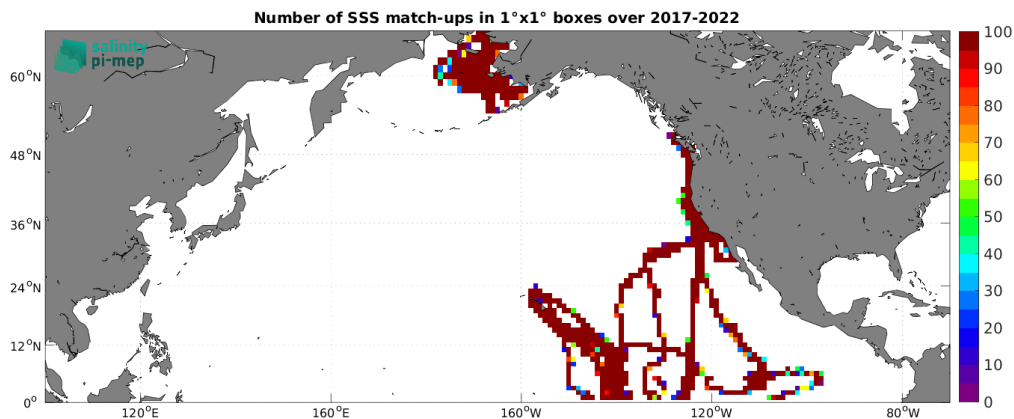
Figure 5: Number of SSS match-ups between Saildrone SSS and the SMAP SSS L3 v5.0 - 8-Day running (JPL) SSS product for the North Pacific Ocean Pi-MEP region over 1^\circ \times 1^\circ boxes and for the full satellite product period.
