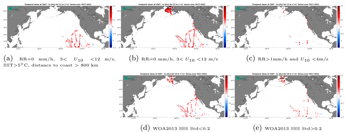
Figure 14: Temporal mean gridded over spatial boxes of size 1^\circ \times 1^\circ of \Delta\text{SSS} (SMAP SSS L3 v5.0 - 8-Day running (JPL) - Sairdrone) for 5 different subdatasets corresponding to: RR=0 mm/h, 3 < U_{10} < 12 m/s, SST > 5°C, distance to coast > 800 km (a), RR=0 mm/h, 3 < U_{10} < 12 m/s (b), RR > 1mm/h and U_{10} < 4 m/s (c), WOA2013 SSS Std < 0.2 (d), WOA2013 SSS Std > 0.2 (e).
