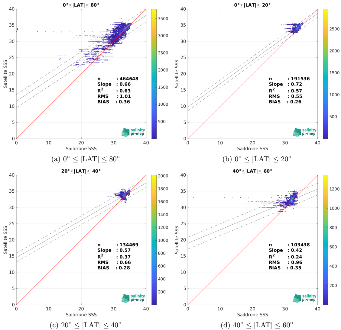
Figure 10: Contour maps of the concentration of SMAP SSS L3 v5.0 - 8-Day running (JPL) SSS (y-axis) versus Sairdrone SSS (x-axis) at match-up pairs for different latitude bands. For each plot, the red line shows x=y . The black thin and dashed lines indicate a linear fit through the data cloud and the \pm 95\% confidence levels, respectively. The number match-up pairs n , the slope and R^2 coefficient of the linear fit, the root mean square (RMS) and the mean bias between satellite and in situ data are indicated for each latitude band in each plots.
