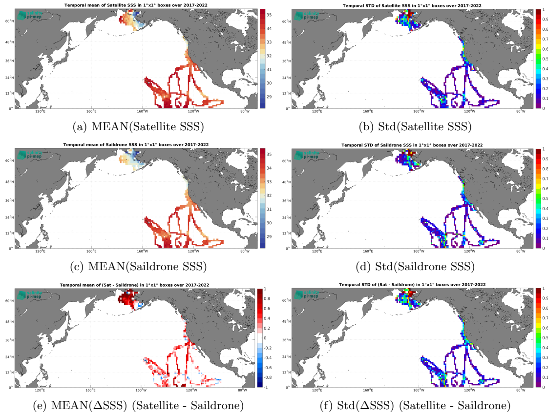
Figure 7: Temporal mean (left) and Std (right) of SSS from SMAP SSS L3 v5.0 - 8-Day running (JPL) (top), Saildrone (middle), and of \Delta SSS (Satellite - Saildrone). Only match-up pairs are used to generate these maps.
