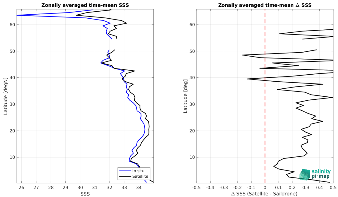
Figure 9: Left panel: Zonal mean SSS from SMAP SSS L3 v5.0 - 8-Day running (JPL) satellite product (black) and from Sairdron (blue). Right panel: Zonal mean of \Delta SSS (Satellite - Sairdron) for all the collected Pi-MEP match-up pairs estimated over the full satellite product period.
