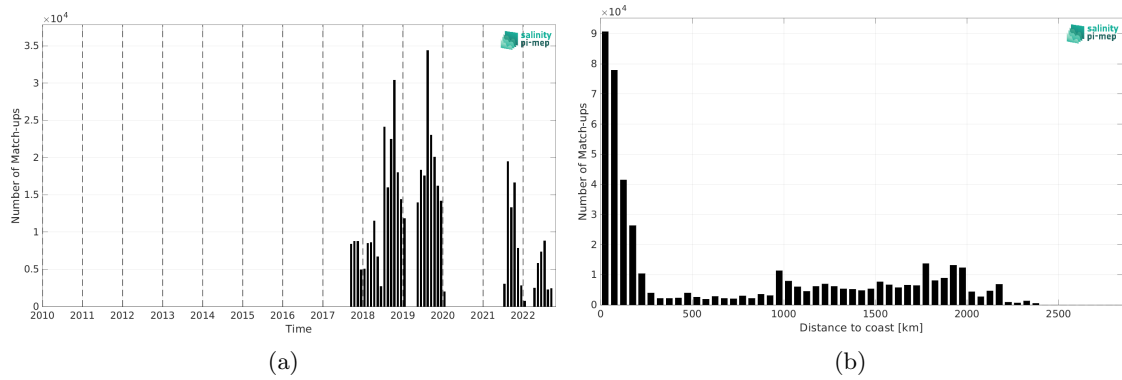
Figure 2: Number of match-ups between Sairdrone and SMAP SSS L3 v5.0 - 8-Day running (JPL) SSS as a function of time (a) and as function of the distance to coast (b) over the North Pacific Ocean Pi-MEP region and for the full satellite product period.
