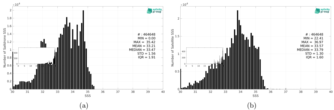
Figure 3: Histograms of SSS from Sairdrone (a) and SMAP SSS L3 v5.0 - 8-Day running (JPL) (b) considering all match-up pairs per bins of 0.1 over the North Pacific Ocean Pi-MEP region and for the full satellite product period.
