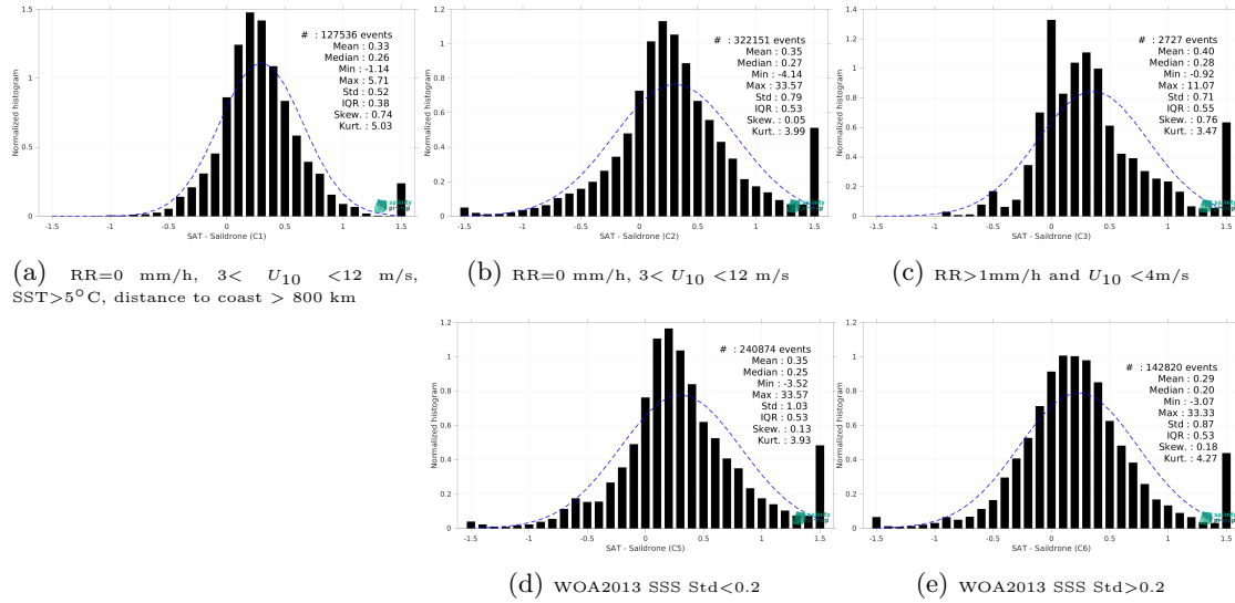
Figure 15: Normalized histogram of \Delta SSS (SMAP SSS L3 v5.0 - 8-Day running (JPL) - Saildrone) for 5 different subdatasets corresponding to: RR=0 mm/h, 3 < U_{10} < 12 m/s, SST>5°C, distance to coast > 800 km (a), RR=0 mm/h, 3 < U_{10} < 12 m/s (b), RR>1mm/h and U_{10} < 4 m/s (c), WOA2013 SSS Std<0.2 (d), WOA2013 SSS Std>0.2 (e).
