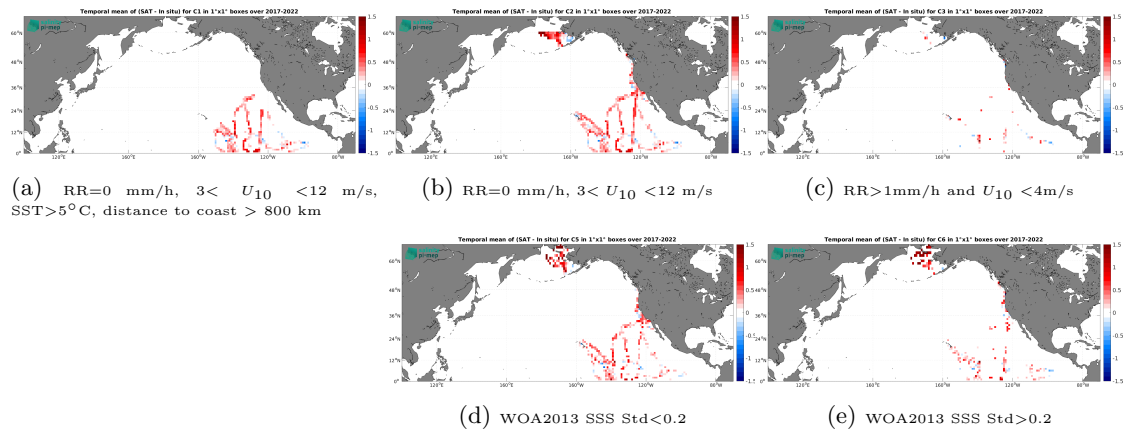
Figure 12: Temporal mean gridded over spatial boxes of size 1^\circ \times 1^\circ of \Delta SSS (SMAP SSS L3 v5.0 - 8-Day running (JPL) - Sairdrone) for 5 different subdatasets corresponding to:RR=0 mm/h, 3 < U_{10} < 12 m/s, SST >5^\circ C, distance to coast > 800 km (a), RR=0 mm/h, 3 < U_{10} < 12 m/s (b), RR >1 mm/h and U_{10} < 4 m/s (c), WOA2013 SSS Std <0.2 (d), WOA2013 SSS Std >0.2 (e).
