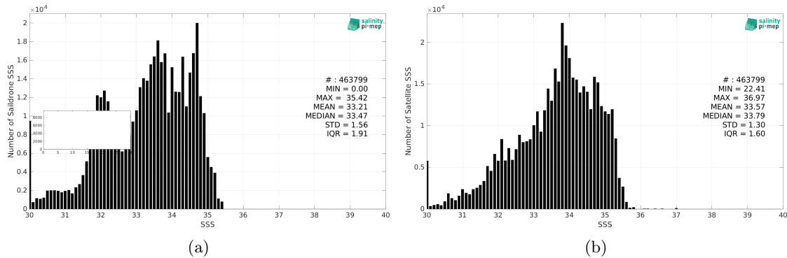
Figure 2: Histograms of SSS from Sairdrone (a) and SMAP SSS L3 v5.0 - 8-Day running (JPL) (b) considering all match-up pairs per bins of 0.1 over the North Pacific Ocean Pi-MEP region and for the full satellite product period.
