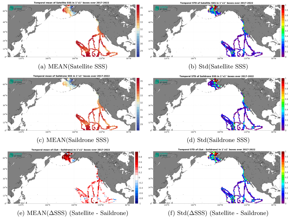
Figure 6: Temporal mean (left) and Std (right) of SSS from SMAP SSS L3 v5.0 - 8-Day running (JPL) (top), Saildrone (middle), and of \Delta SSS (Satellite - Saildrone). Only match-up pairs are used to generate these maps.
