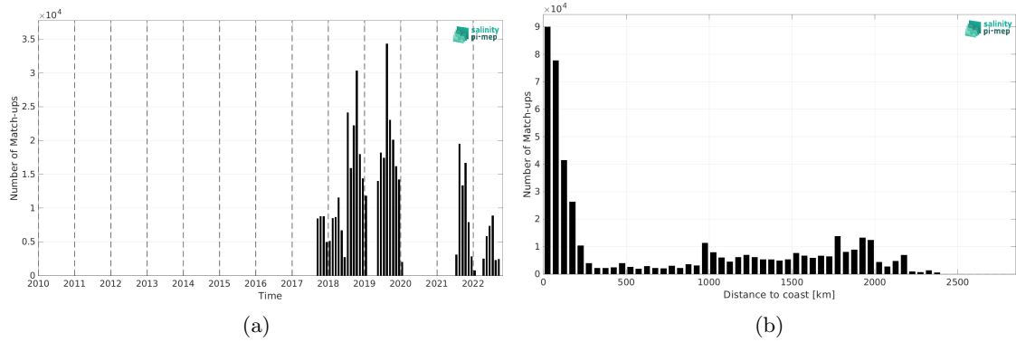
Figure 1: Number of match-ups between Sairdrone and SMAP SSS L3 v5.0 - 8-Day running (JPL) SSS as a function of time (a) and as function of the distance to coast (b) over the North Pacific Ocean Pi-MEP region and for the full satellite product period.
