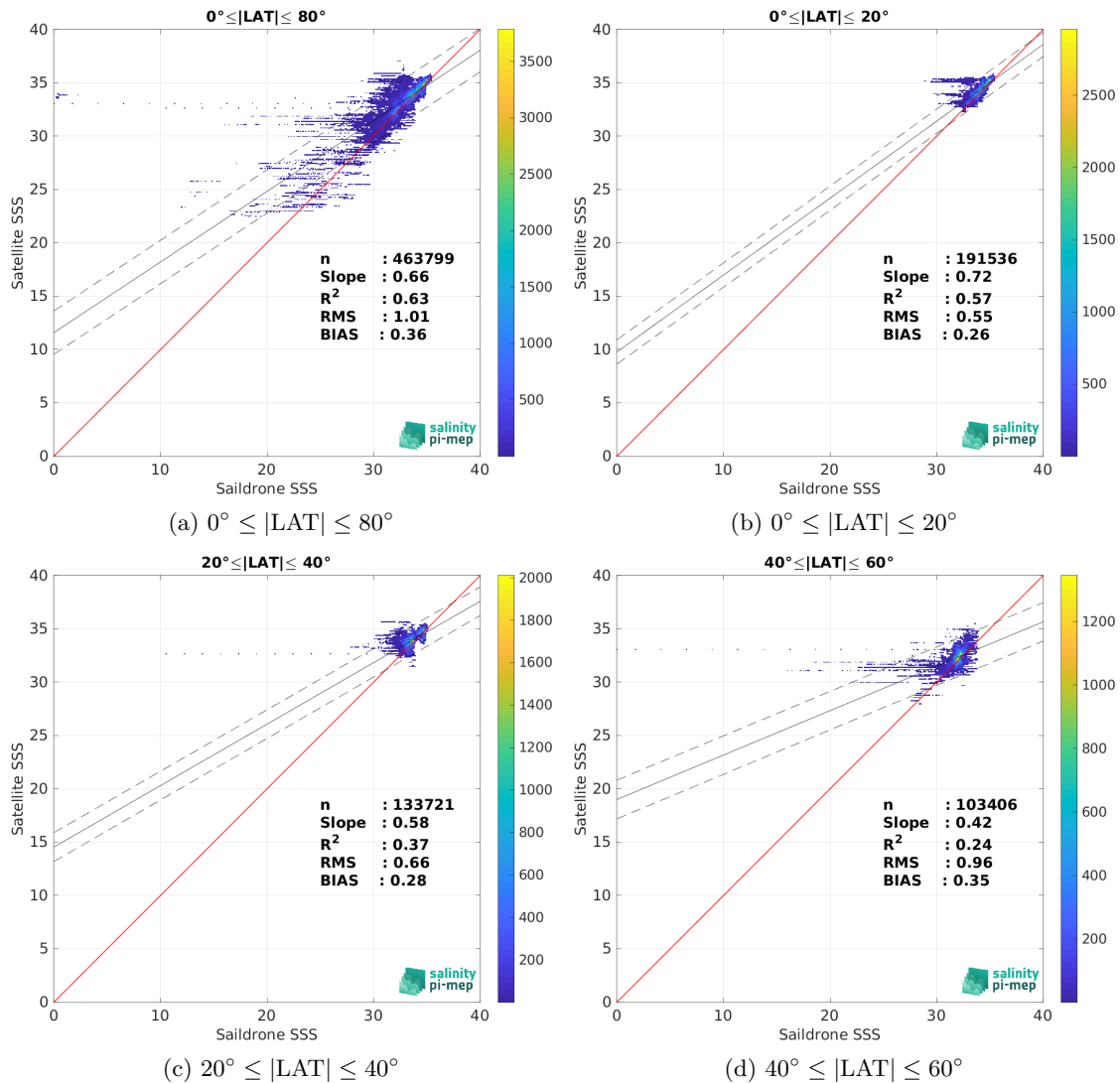
Figure 9: Contour maps of the concentration of SMAP SSS L3 v5.0 - 8-Day running (JPL) SSS (y-axis) versus Saildrone SSS (x-axis) at match-up pairs for different latitude bands. For each plot, the red line shows x=y . The black thin and dashed lines indicate a linear fit through the data cloud and the \pm 95\% confidence levels, respectively. The number match-up pairs n , the slope and R^2 coefficient of the linear fit, the root mean square (RMS) and the mean bias between satellite and in situ data are indicated for each latitude band in each plots.
