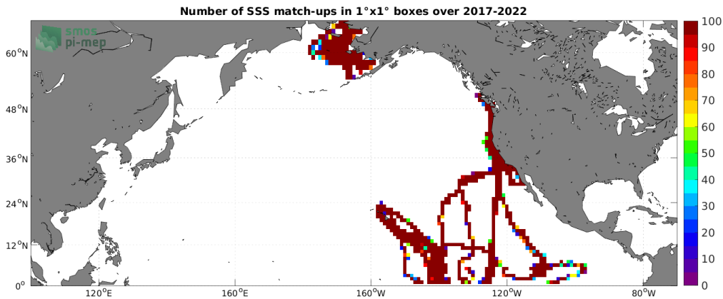
Figure 4: Number of SSS match-ups between Saildrone SSS and the SMAP SSS L3 v5.0 - 8-Day running (JPL) SSS product for the North Pacific Ocean Pi-MEP region over 1^\circ \times 1^\circ boxes and for the full satellite product period.
