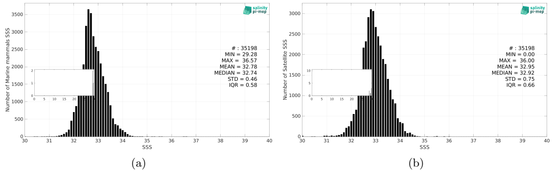
Figure 3: Histograms of SSS from Marine mammals (a) and SMAP SSS L3 v5.0 - 8-Day running (JPL) (b) considering all match-up pairs per bins of 0.1 over the North Pacific Ocean Pi-MEP region and for the full satellite product period.
