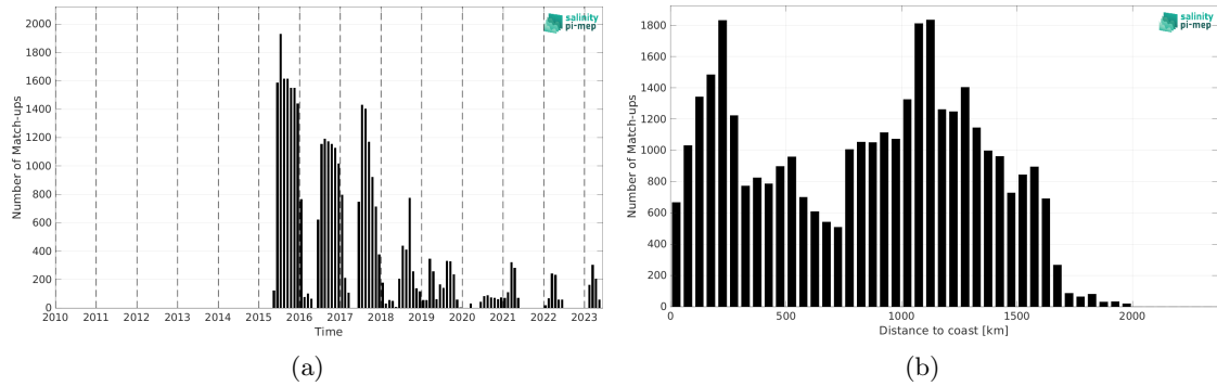
Figure 2: Number of match-ups between Marine mammals and SMAP SSS L3 v5.0 - 8-Day running (JPL) SSS as a function of time (a) and as function of the distance to coast (b) over the North Pacific Ocean Pi-MEP region and for the full satellite product period.
