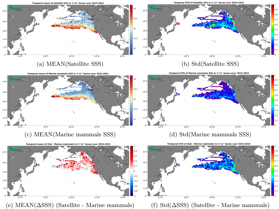
Figure 7: Temporal mean (left) and Std (right) of SSS from SMAP SSS L3 v5.0 - 8-Day running (JPL) (top), Marine mammals (middle), and of \Delta SSS (Satellite - Marine mammals). Only match-up pairs are used to generate these maps.
