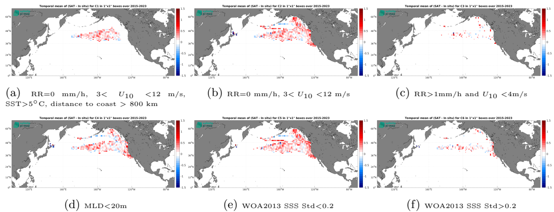
Figure 14: Temporal mean gridded over spatial boxes of size 1^\circ \times 1^\circ of \Delta SSS (SMAP SSS L3 v5.0 - 8-Day running (JPL) - Marine mammals) for 6 different subdatasets corresponding to:RR=0 mm/h, 3 < U_{10} < 12 m/s, SST >5^\circ C, distance to coast > 800 km (a), RR=0 mm/h, 3 < U_{10} < 12 m/s (b), RR >1 mm/h and U_{10} < 4 m/s (c),MLD <20 m (d),WOA2013 SSS Std <0.2 (e),WOA2013 SSS Std >0.2 (f).
