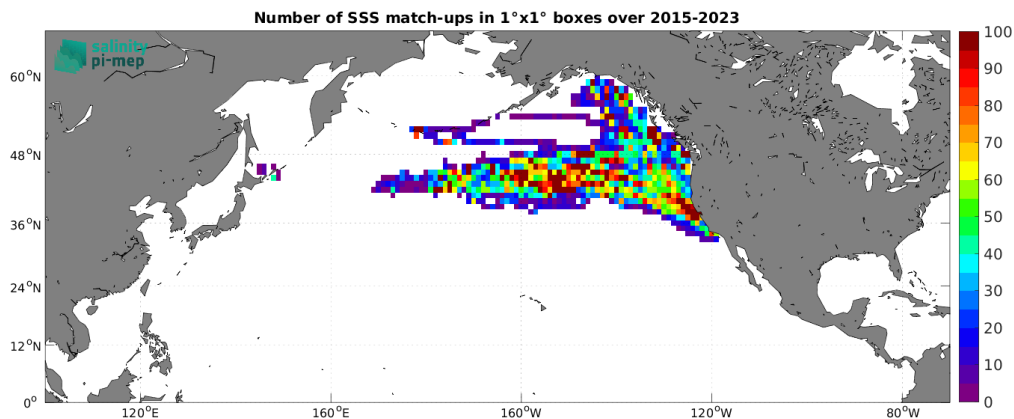
Figure 5: Number of SSS match-ups between Marine mammals SSS and the SMAP SSS L3 v5.0 - 8-Day running (JPL) SSS product for the North Pacific Ocean Pi-MEP region over 1^\circ \times 1^\circ boxes and for the full satellite product period.
