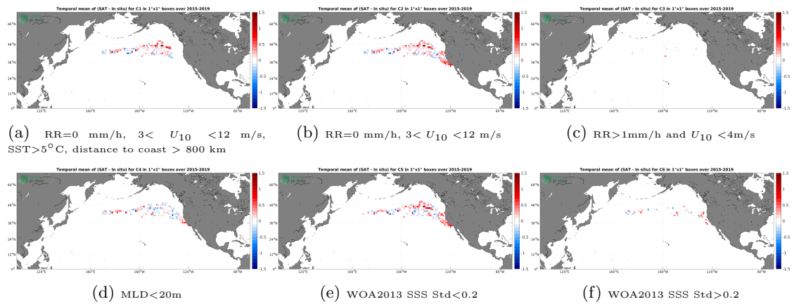
Figure 12: Temporal mean gridded over spatial boxes of size 1^\circ \times 1^\circ of \Delta SSS (SMAP SSS L3 v5.0 - 8-Day running (JPL) - Marine mammals) for 6 different subdatasets corresponding to:RR=0 mm/h, 3 < U_{10} < 12 m/s, SST >5^\circ C, distance to coast > 800 km (a), RR=0 mm/h, 3 < U_{10} < 12 m/s (b), RR >1 mm/h and U_{10} < 4 m/s (c),MLD <20 m (d),WOA2013 SSS Std <0.2 (e),WOA2013 SSS Std >0.2 (f).
