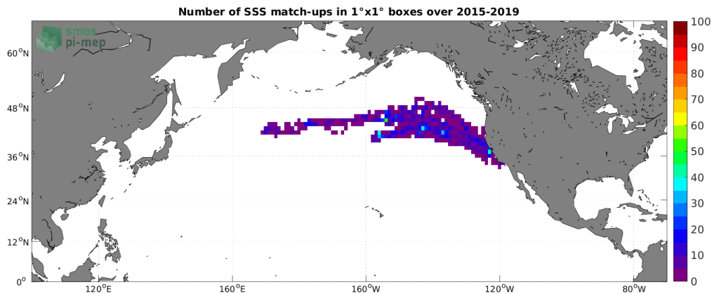
Figure 4: Number of SSS match-ups between Marine mammals SSS and the SMAP SSS L3 v5.0 - 8-Day running (JPL) SSS product for the North Pacific Ocean Pi-MEP region over 1^\circ \times 1^\circ boxes and for the full satellite product period.
