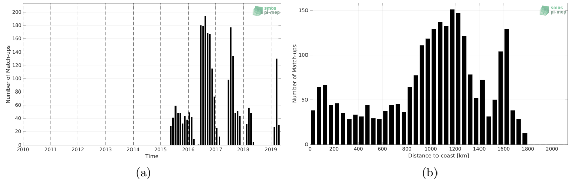
Figure 1: Number of match-ups between Marine mammals and SMAP SSS L3 v5.0 - 8-Day running (JPL) SSS as a function of time (a) and as function of the distance to coast (b) over the North Pacific Ocean Pi-MEP region and for the full satellite product period.
