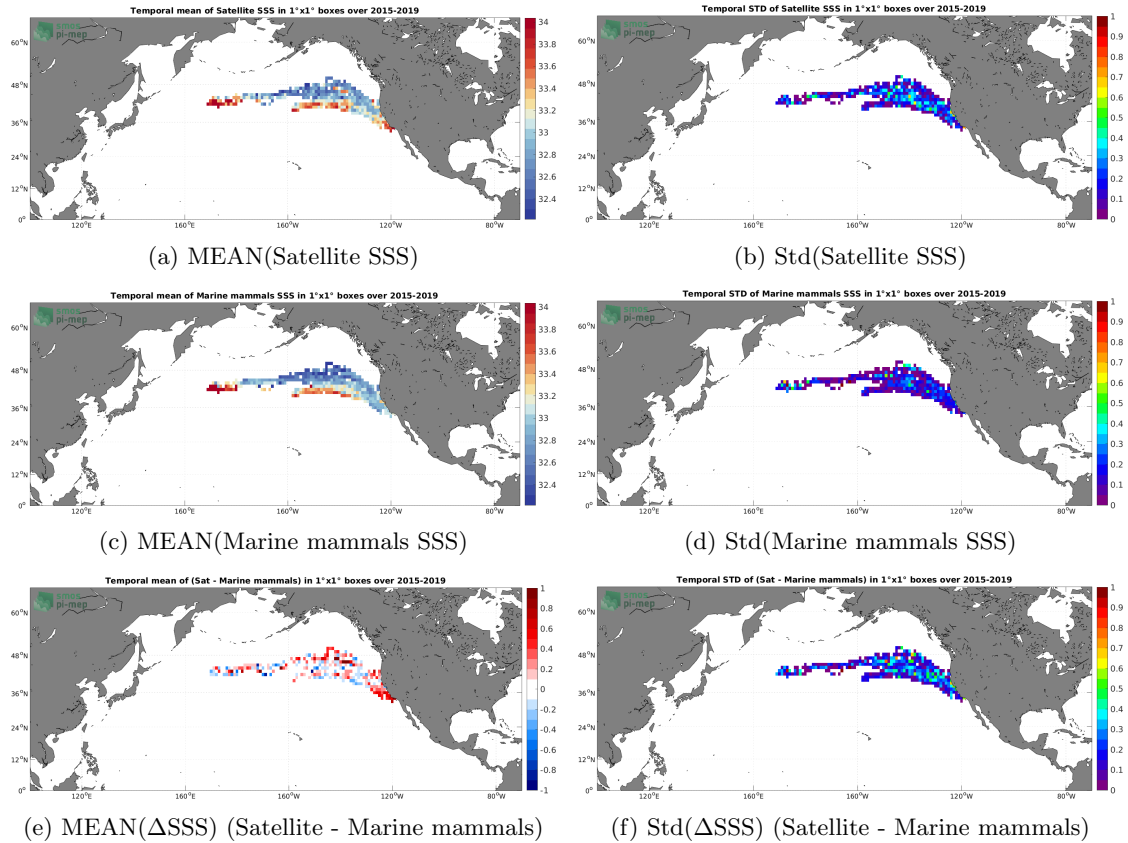
Figure 6: Temporal mean (left) and Std (right) of SSS from SMAP SSS L3 v5.0 - 8-Day running (JPL) (top), Marine mammals (middle), and of \Delta SSS (Satellite - Marine mammals). Only match-up pairs are used to generate these maps.
