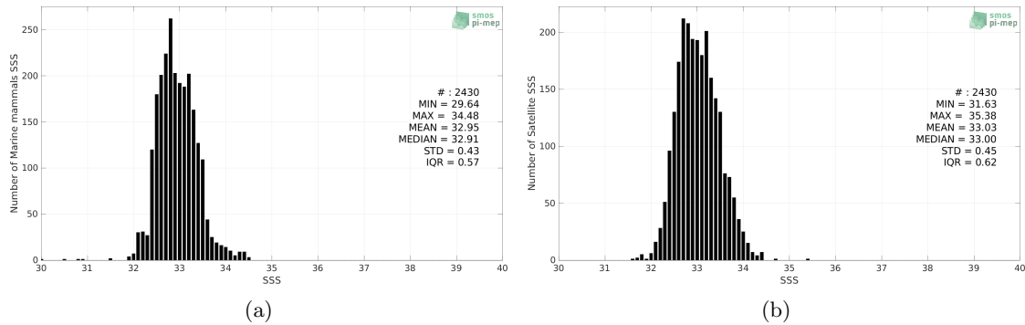
Figure 2: Histograms of SSS from Marine mammals (a) and SMAP SSS L3 v5.0 - 8-Day running (JPL) (b) considering all match-up pairs per bins of 0.1 over the North Pacific Ocean Pi-MEP region and for the full satellite product period.
