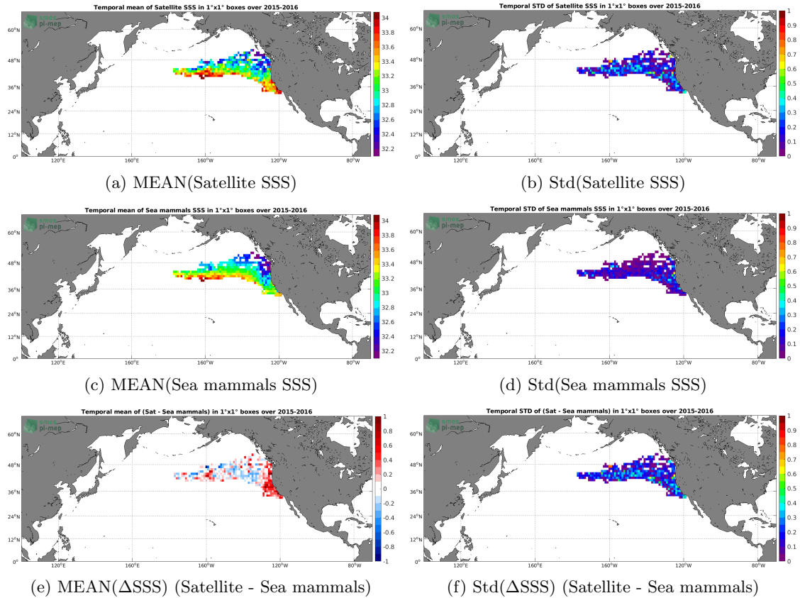
Figure 6: Temporal mean (left) and Std (right) of SSS from SMAP SSS L3 v5.0 - 8-Day running (JPL) (top), Sea mammals (middle), and of \Delta\text{SSS} (Satellite - Sea mammals). Only match-up pairs are used to generate these maps.
