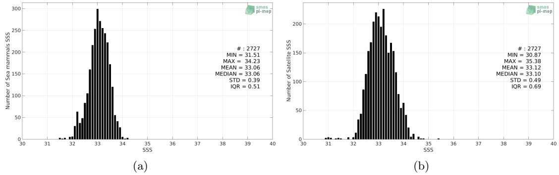
Figure 2: Histograms of SSS from Sea mammals (a) and SMAP SSS L3 v5.0 - 8-Day running (JPL) (b) considering all match-up pairs per bins of 0.1 over the North Pacific Ocean Pi-MEP region and for the full satellite product period.
