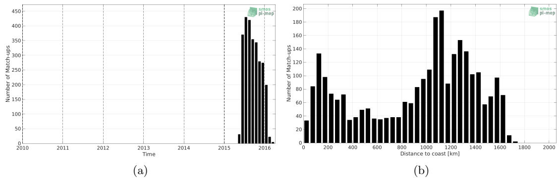
Figure 1: Number of match-ups between Sea mammals and SMAP SSS L3 v5.0 - 8-Day running (JPL) SSS as a function of time (a) and as function of the distance to coast (b) over the North Pacific Ocean Pi-MEP region and for the full satellite product period.
