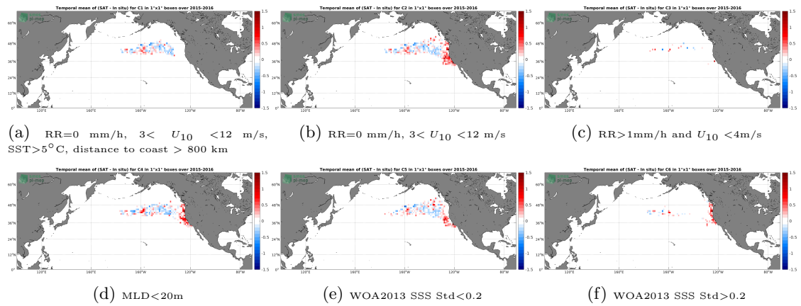
Figure 12: Temporal mean gridded over spatial boxes of size 1°x1° of \Delta SSS (SMAP SSS L3 v5.0 - 8-Day running (JPL) - Sea mammals) for 6 different subdatasets corresponding to:RR=0 mm/h, 3 < U_{10} < 12 m/s, SST>5°C, distance to coast > 800 km (a), RR=0 mm/h, 3 < U_{10} < 12 m/s (b), RR>1mm/h and U_{10} < 4 m/s (c),MLD<20m (d),WOA2013 SSS Std<0.2 (e),WOA2013 SSS Std>0.2 (f).
