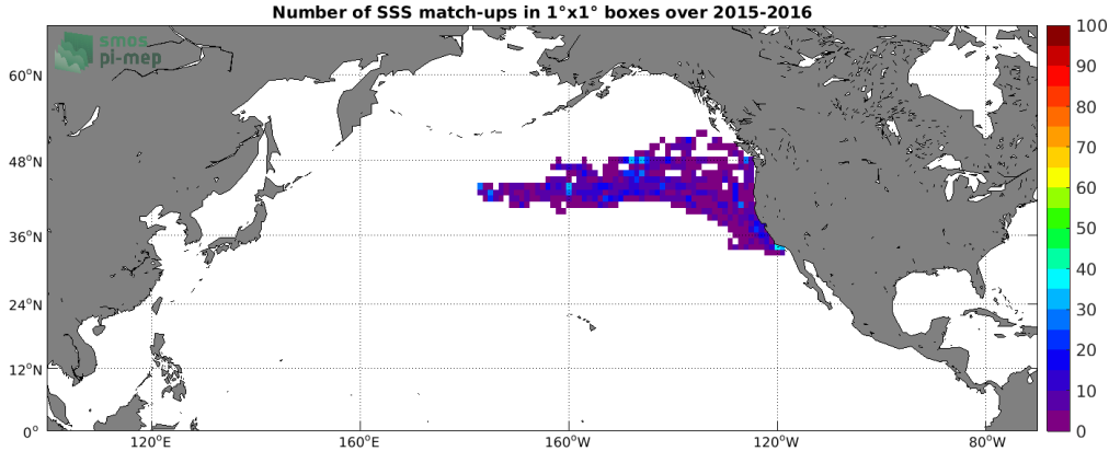
Figure 4: Number of SSS match-ups between Sea mammals SSS and the SMAP SSS L3 v5.0 - 8-Day running (JPL) SSS product for the North Pacific Ocean Pi-MEP region over 1^\circ \times 1^\circ boxes and for the full satellite product period.
