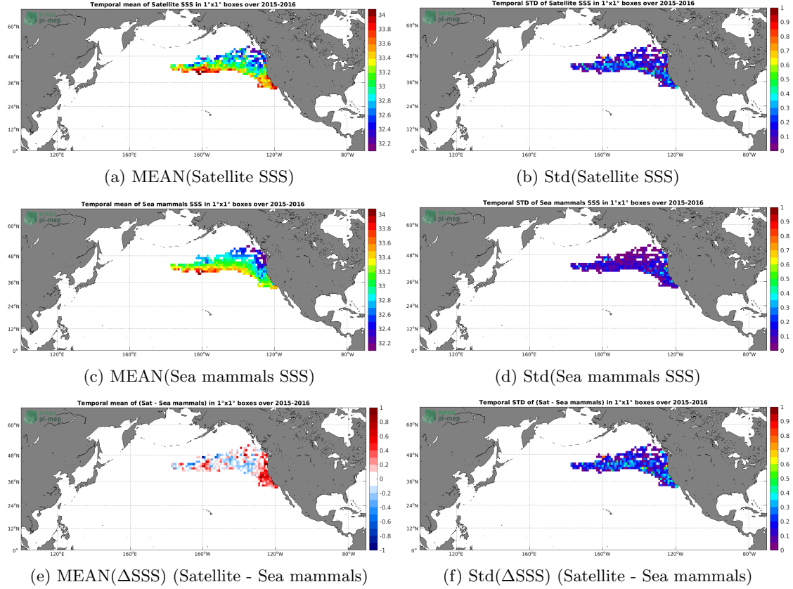
Figure 6: Temporal mean (left) and Std (right) of SSS from SMAP SSS L3 v5.0 - 8-Day running (JPL) (top), Sea mammals (middle), and of \Delta SSS (Satellite - Sea mammals). Only match-up pairs are used to generate these maps.
