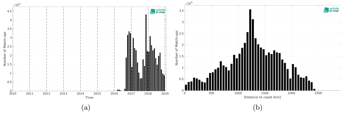
Figure 2: Number of match-ups between Surface drifters and SMAP SSS L3 v5.0 - 8-Day running (JPL) SSS as a function of time (a) and as function of the distance to coast (b) over the North Pacific Ocean Pi-MEP region and for the full satellite product period.
