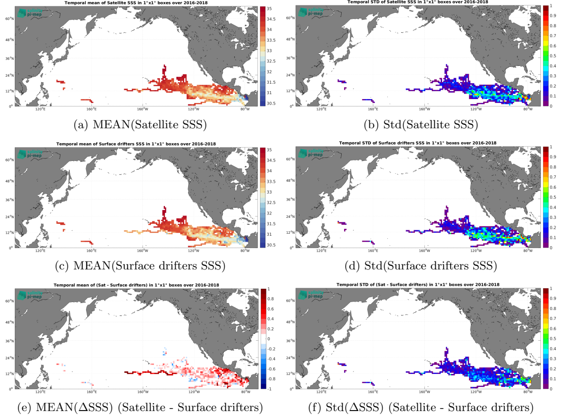
Figure 6: Temporal mean (left) and Std (right) of SSS from SMAP SSS L3 v5.0 - 8-Day running (JPL) (top), Surface drifters (middle), and of \Delta SSS (Satellite - Surface drifters). Only match-up pairs are used to generate these maps.
