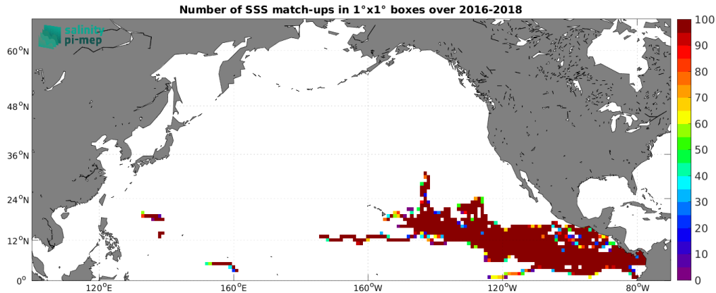
Figure 4: Number of SSS match-ups between Surface drifters SSS and the SMAP SSS L3 v5.0 - 8-Day running (JPL) SSS product for the North Pacific Ocean Pi-MEP region over 1^\circ \times 1^\circ boxes and for the full satellite product period.
