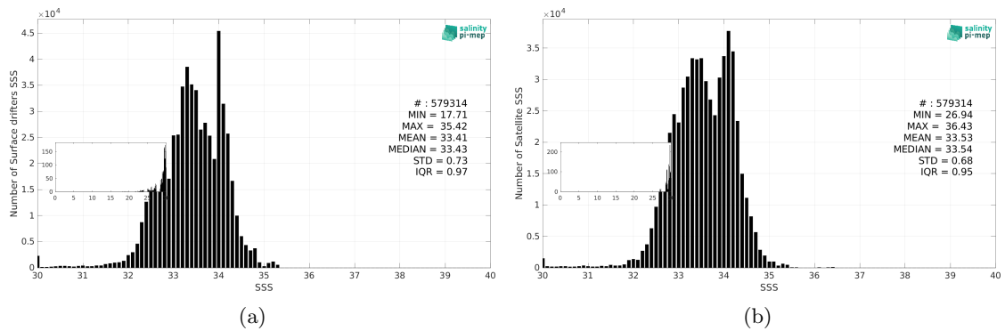
Figure 3: Histograms of SSS from Surface drifters (a) and SMAP SSS L3 v5.0 - 8-Day running (JPL) (b) considering all match-up pairs per bins of 0.1 over the North Pacific Ocean Pi-MEP region and for the full satellite product period.
