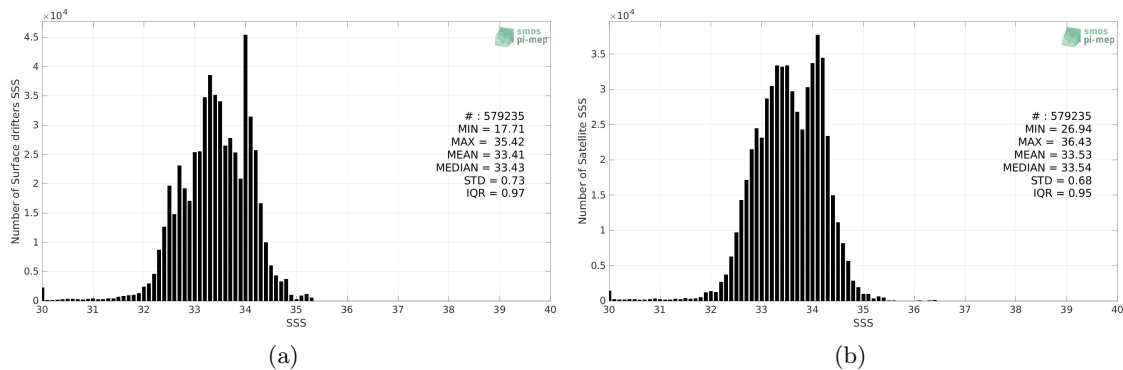
Figure 2: Histograms of SSS from Surface drifters (a) and SMAP SSS L3 v5.0 - 8-Day running (JPL) (b) considering all match-up pairs per bins of 0.1 over the North Pacific Ocean Pi-MEP region and for the full satellite product period.
