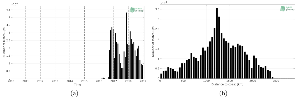
Figure 1: Number of match-ups between Surface drifters and SMAP SSS L3 v5.0 - 8-Day running (JPL) SSS as a function of time (a) and as function of the distance to coast (b) over the North Pacific Ocean Pi-MEP region and for the full satellite product period.
