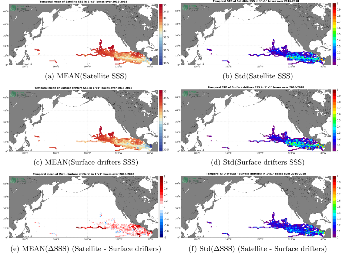
Figure 5: Temporal mean (left) and Std (right) of SSS from SMAP SSS L3 v5.0 - 8-Day running (JPL) (top), Surface drifters (middle), and of \Delta SSS (Satellite - Surface drifters). Only match-up pairs are used to generate these maps.
