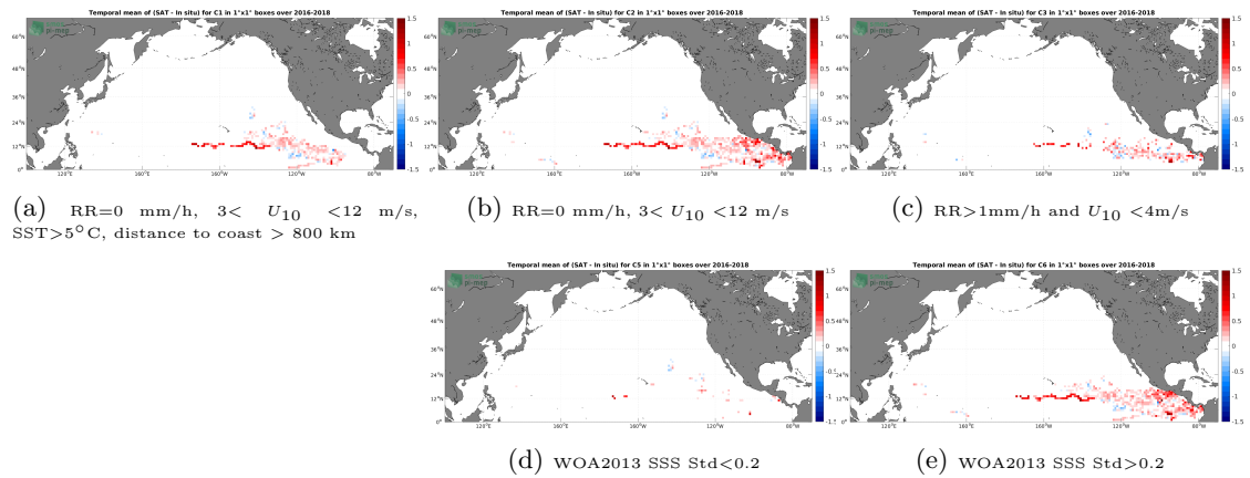
Figure 11: Temporal mean gridded over spatial boxes of size 1^\circ \times 1^\circ of \Delta SSS (SMAP SSS L3 v5.0 - 8-Day running (JPL) - Surface drifters) for 5 different subdatasets corresponding to:RR=0 mm/h, 3 < U_{10} < 12 m/s, SST >5^\circ C, distance to coast > 800 km (a), RR=0 mm/h, 3 < U_{10} < 12 m/s (b), RR >1 mm/h and U_{10} < 4 m/s (c), WOA2013 SSS Std <0.2 (d), WOA2013 SSS Std >0.2 (e).
