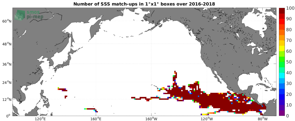
Figure 3: Number of SSS match-ups between Surface drifters SSS and the SMAP SSS L3 v5.0 - 8-Day running (JPL) SSS product for the North Pacific Ocean Pi-MEP region over 1^\circ \times 1^\circ boxes and for the full satellite product period.
