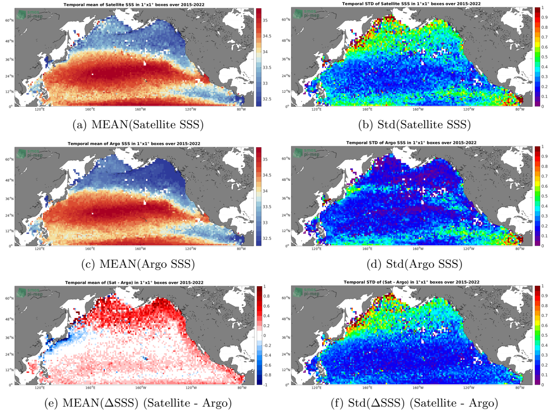
Figure 6: Temporal mean (left) and Std (right) of SSS from SMAP SSS L3 v5.0 - 8-Day running (JPL) (top), Argo (middle), and of \Delta\text{SSS} (Satellite - Argo). Only match-up pairs are used to generate these maps.
