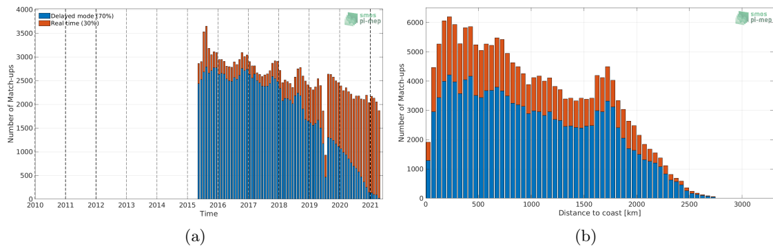
Figure 1: Number of match-ups between Argo and SMAP SSS L3 v5.0 - 8-Day running (JPL) SSS as a function of time (a) and as function of the distance to coast (b) over the North Pacific Ocean Pi-MEP region and for the full satellite product period.
