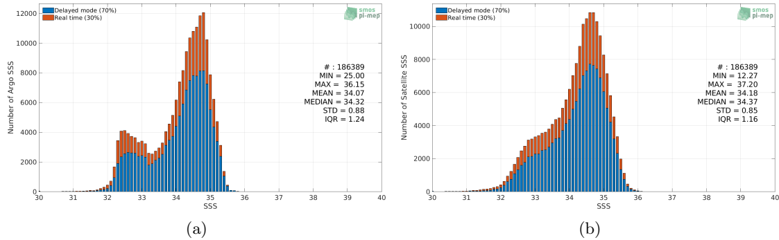
Figure 2: Histograms of SSS from Argo (a) and SMAP SSS L3 v5.0 - 8-Day running (JPL) (b) considering all match-up pairs per bins of 0.1 over the North Pacific Ocean Pi-MEP region and for the full satellite product period.
