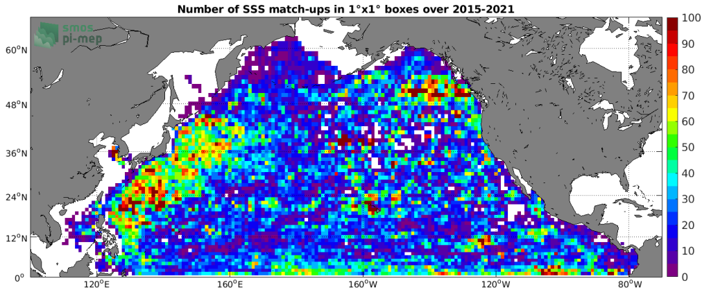
Figure 4: Number of SSS match-ups between Argo SSS and the SMAP SSS L3 v5.0 - 8-Day running (JPL) SSS product for the North Pacific Ocean Pi-MEP region over 1^\circ \times 1^\circ boxes and for the full satellite product period.
