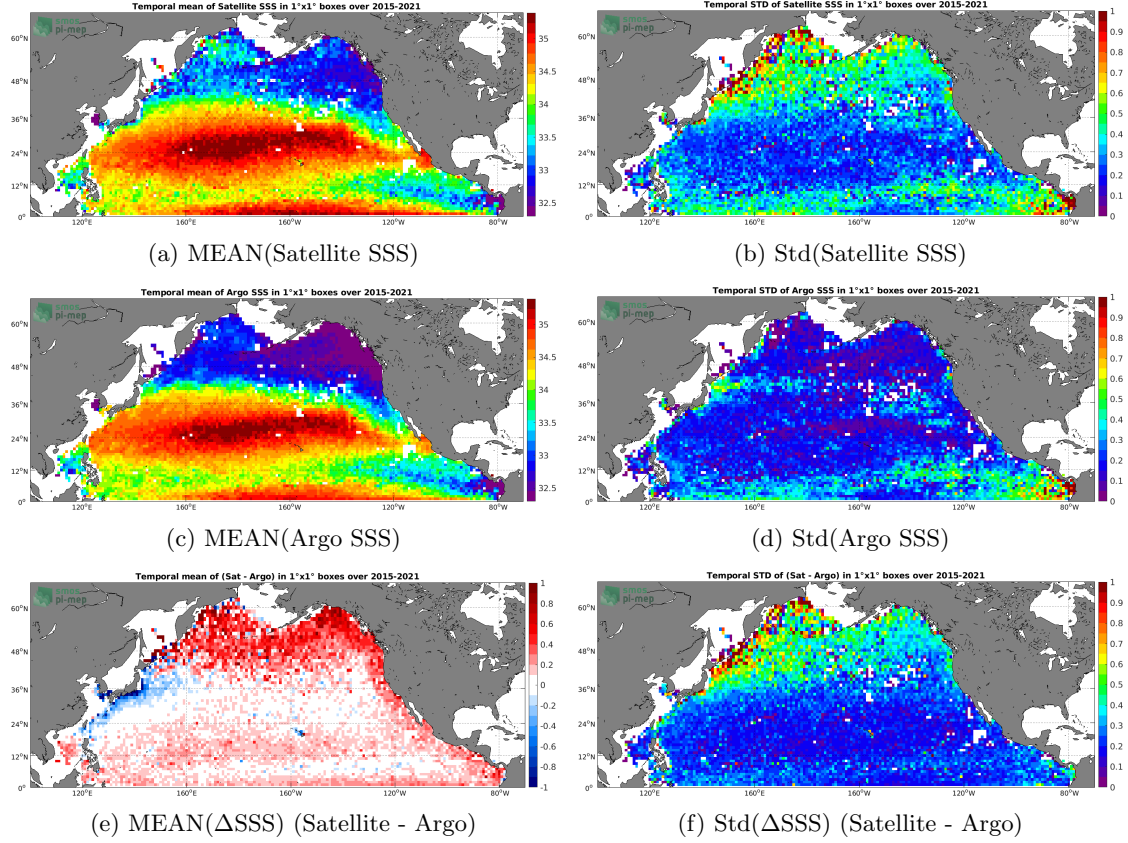
Figure 6: Temporal mean (left) and Std (right) of SSS from SMAP SSS L3 v5.0 - 8-Day running (JPL) (top), Argo (middle), and of \Delta SSS (Satellite - Argo). Only match-up pairs are used to generate these maps.
