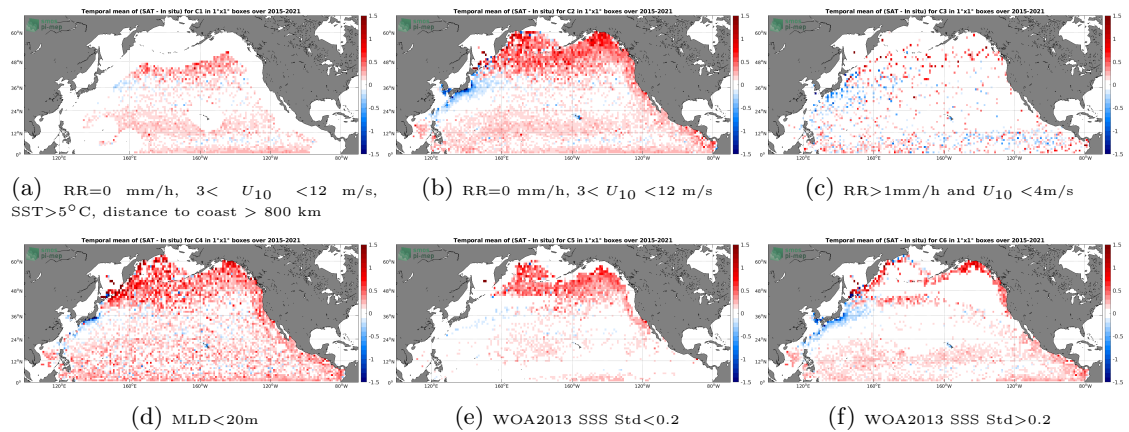
Figure 12: Temporal mean gridded over spatial boxes of size 1^\circ \times 1^\circ of \Delta SSS (SMAP SSS L3 v5.0 - 8-Day running (JPL) - Argo) for 6 different subdatasets corresponding to:RR=0 mm/h, 3 < U_{10} < 12 m/s, SST > 5^\circ C , distance to coast > 800 km (a), RR=0 mm/h, 3 < U_{10} < 12 m/s (b), RR>1mm/h and U_{10} < 4 m/s (c),MLD<20m (d),WOA2013 SSS Std<0.2 (e),WOA2013 SSS Std>0.2 (f).
