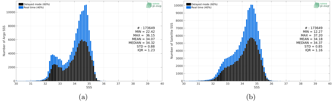
Figure 2: Histograms of SSS from Argo (a) and SMAP SSS L3 v5.0 - 8-Day running (JPL) (b) considering all match-up pairs per bins of 0.1 over the North Pacific Ocean Pi-MEP region and for the full satellite product period.
