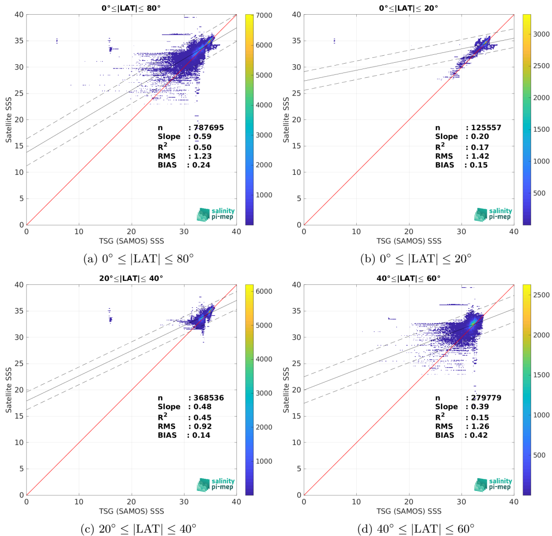
Figure 9: Contour maps of the concentration of SMAP SSS L3 v5.0 - Monthly (JPL) SSS (y-axis) versus TSG (SAMOS) SSS (x-axis) at match-up pairs for different latitude bands. For each plot, the red line shows x=y . The black thin and dashed lines indicate a linear fit through the data cloud and the \pm 95\% confidence levels, respectively. The number match-up pairs n , the slope and R^2 coefficient of the linear fit, the root mean square (RMS) and the mean bias between satellite and in situ data are indicated for each latitude band in each plots.
