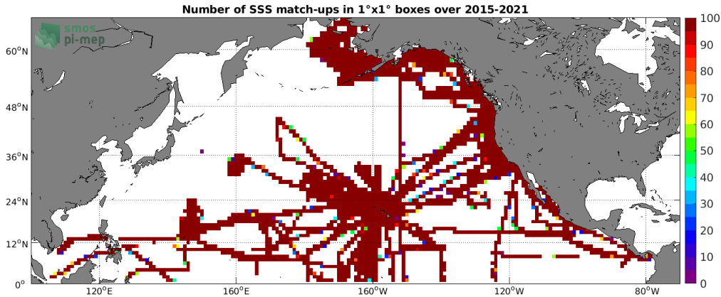
Figure 4: Number of SSS match-ups between TSG (SAMOS) SSS and the SMAP SSS L3 v5.0 - Monthly (JPL) SSS product for the North Pacific Ocean Pi-MEP region over 1°x1° boxes and for the full satellite product period.
