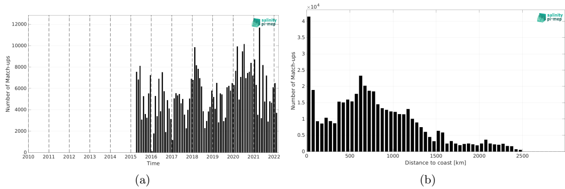
Figure 2: Number of match-ups between TSG (LEGOS-DM) and SMAP SSS L3 v5.0 - Monthly (JPL) SSS as a function of time (a) and as function of the distance to coast (b) over the North Pacific Ocean Pi-MEP region and for the full satellite product period.
