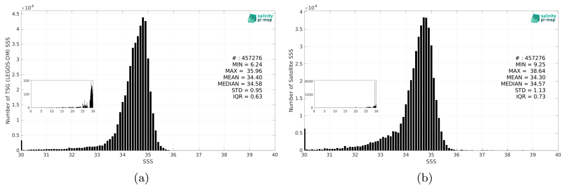
Figure 3: Histograms of SSS from TSG (LEGOS-DM) (a) and SMAP SSS L3 v5.0 - Monthly (JPL) (b) considering all match-up pairs per bins of 0.1 over the North Pacific Ocean Pi-MEP region and for the full satellite product period.
