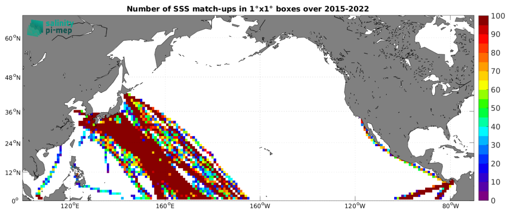
Figure 5: Number of SSS match-ups between TSG (LEGOS-DM) SSS and the SMAP SSS L3 v5.0 - Monthly (JPL) SSS product for the North Pacific Ocean Pi-MEP region over 1^\circ \times 1^\circ boxes and for the full satellite product period.
