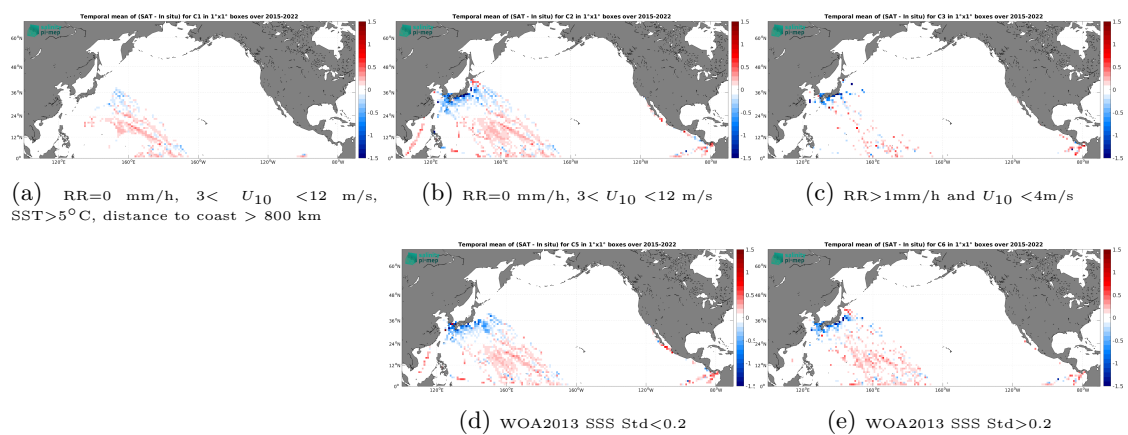
Figure 14: Temporal mean gridded over spatial boxes of size 1^\circ \times 1^\circ of \Delta\text{SSS} (SMAP SSS L3 v5.0 - Monthly (JPL) - TSG (LEGOS-DM)) for 5 different subdatasets corresponding to: RR=0 mm/h, 3 < U_{10} < 12 m/s, SST > 5°C, distance to coast > 800 km (a), RR=0 mm/h, 3 < U_{10} < 12 m/s (b), RR > 1mm/h and U_{10} < 4 m/s (c), WOA2013 SSS Std < 0.2 (d), WOA2013 SSS Std > 0.2 (e).
