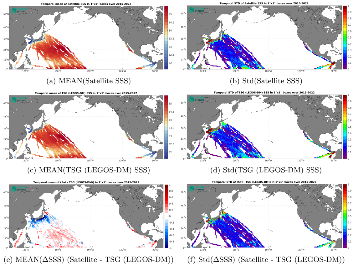
Figure 7: Temporal mean (left) and Std (right) of SSS from SMAP SSS L3 v5.0 - Monthly (JPL) (top), TSG (LEGOS-DM) (middle), and of \Delta SSS (Satellite - TSG (LEGOS-DM)). Only match-up pairs are used to generate these maps.
