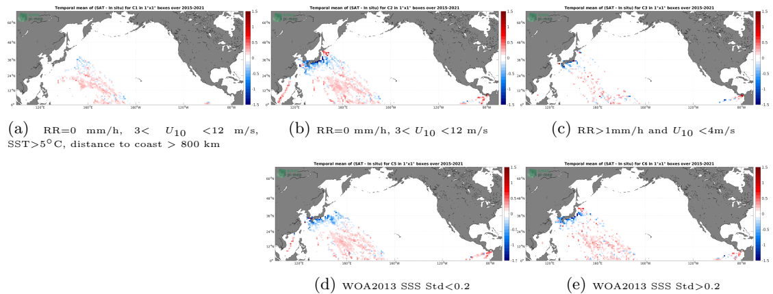
Figure 12: Temporal mean gridded over spatial boxes of size 1^\circ \times 1^\circ of \Delta SSS (SMAP SSS L3 v5.0 - Monthly (JPL) - TSG (LEGOS-DM)) for 5 different subdatasets corresponding to:RR=0 mm/h, 3 < U_{10} < 12 m/s, SST > 5^\circ C , distance to coast > 800 km (a), RR=0 mm/h, 3 < U_{10} < 12 m/s (b), RR >1 mm/h and U_{10} < 4 m/s (c), WOA2013 SSS Std <0.2 (d), WOA2013 SSS Std >0.2 (e).
