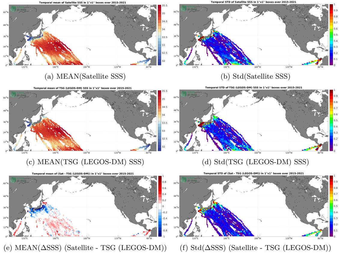
Figure 6: Temporal mean (left) and Std (right) of SSS from SMAP SSS L3 v5.0 - Monthly (JPL) (top), TSG (LEGOS-DM) (middle), and of \Delta SSS (Satellite - TSG (LEGOS-DM)). Only match-up pairs are used to generate these maps.
