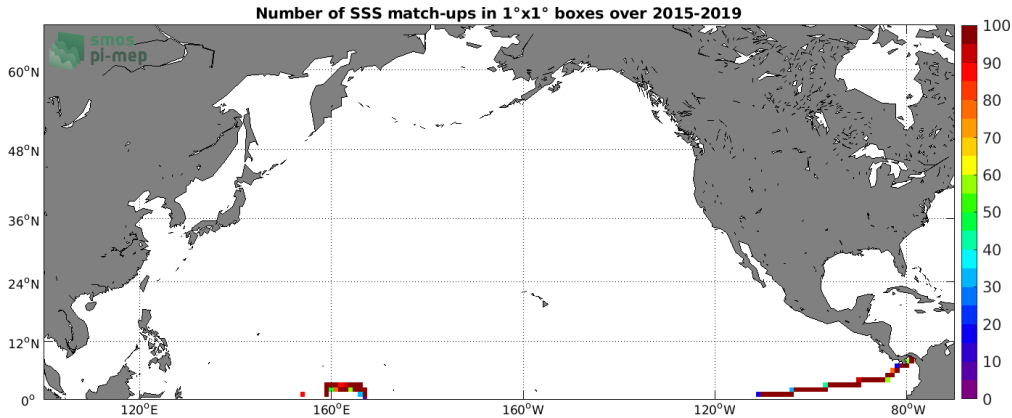
Figure 4: Number of SSS match-ups between TSG (GOSUD-Research-vessel) SSS and the SMAP SSS L3 v5.0 - Monthly (JPL) SSS product for the North Pacific Ocean Pi-MEP region over 1°x1° boxes and for the full satellite product period.
