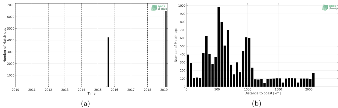
Figure 1: Number of match-ups between TSG (GOSUD-Research-vessel) and SMAP SSS L3 v5.0 - Monthly (JPL) SSS as a function of time (a) and as function of the distance to coast (b) over the North Pacific Ocean Pi-MEP region and for the full satellite product period.
