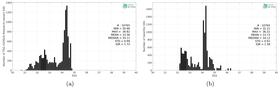
Figure 2: Histograms of SSS from TSG (GOSUD-Research-vessel) (a) and SMAP SSS L3 v5.0 - Monthly (JPL) (b) considering all match-up pairs per bins of 0.1 over the North Pacific Ocean Pi-MEP region and for the full satellite product period.
