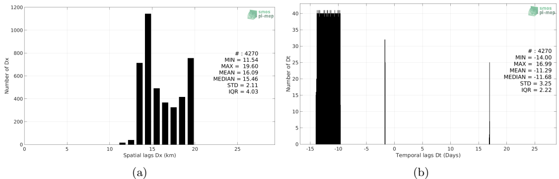
Figure 5: Histograms of the spatial (a) and temporal (b) lags between the time of the TSG (GOSUD-Research-vessel) measurements and the date of the corresponding SMAP SSS L3 v5.0 - Monthly (JPL) SSS product.
