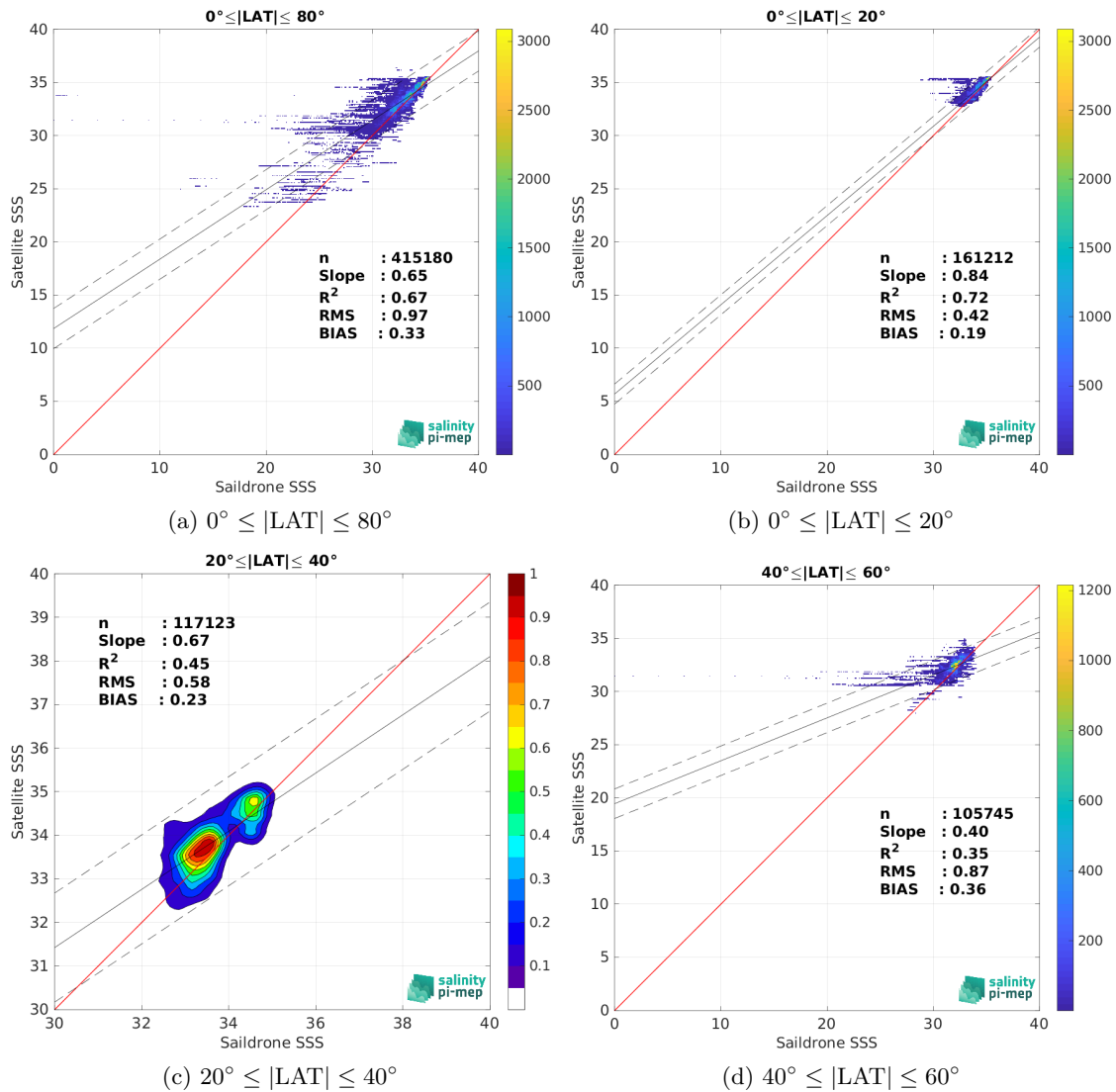
Figure 10: Contour maps of the concentration of SMAP SSS L3 v5.0 - Monthly (JPL) SSS (y-axis) versus Sairdrone SSS (x-axis) at match-up pairs for different latitude bands. For each plot, the red line shows x=y . The black thin and dashed lines indicate a linear fit through the data cloud and the \pm 95\% confidence levels, respectively. The number match-up pairs n , the slope and R^2 coefficient of the linear fit, the root mean square (RMS) and the mean bias between satellite and in situ data are indicated for each latitude band in each plots.
