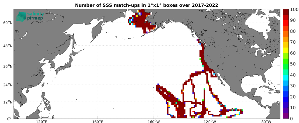
Figure 4: Number of SSS match-ups between Ssaldrone SSS and the SMAP SSS L3 v5.0 - Monthly (JPL) SSS product for the North Pacific Ocean Pi-MEP region over 1^\circ \times 1^\circ boxes and for the full satellite product period.
