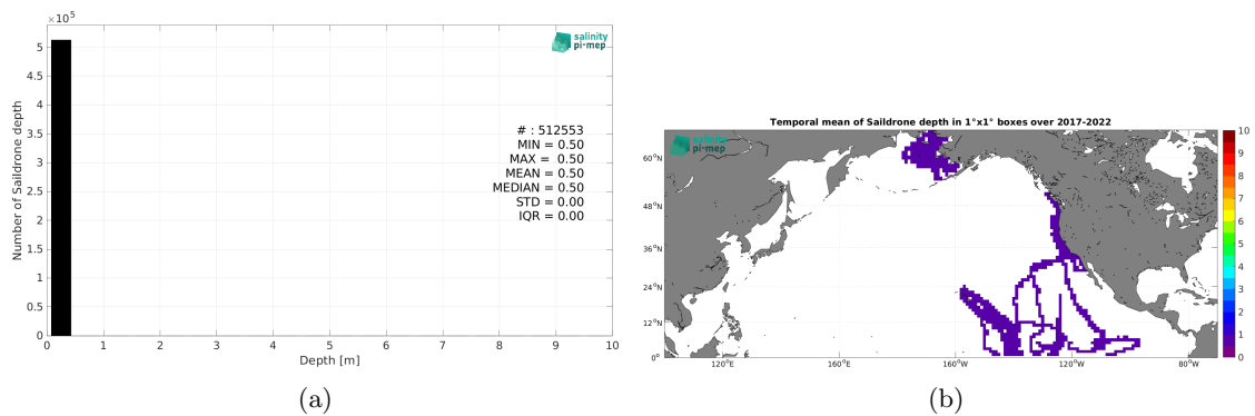
Figure 3: Histograms of the depth of the upper level SSS measurements from Ssaldrone in the Match-up DataBase for the North Pacific Ocean Pi-MEP region (a) and temporal mean spatial distribution of pressure of the in situ SSS data over 1^\circ \times 1^\circ boxes and for the full satellite product period (b).
