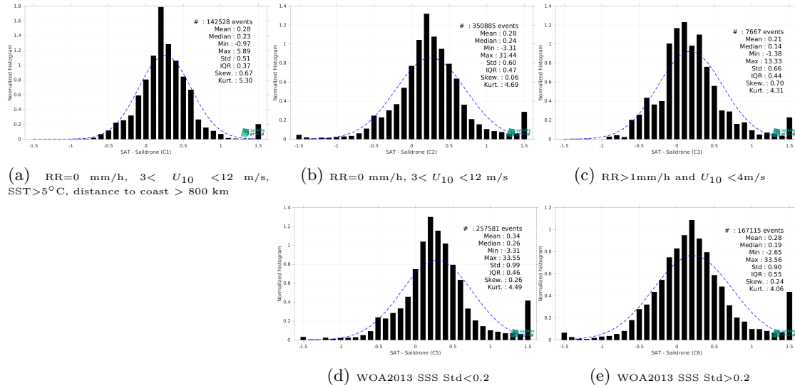
Figure 13: Normalized histogram of \Delta SSS (SMAP SSS L3 v5.0 - Monthly (JPL) - Saildrone) for 5 different subdatasets corresponding to: RR=0 mm/h, 3 < U_{10} < 12 m/s, SST >5^{\circ} C, distance to coast > 800 km (a), RR=0 mm/h, 3 < U_{10} < 12 m/s (b), RR >1 mm/h and U_{10} < 4 m/s (c), WOA2013 SSS Std <0.2 (d), WOA2013 SSS Std >0.2 (e).
