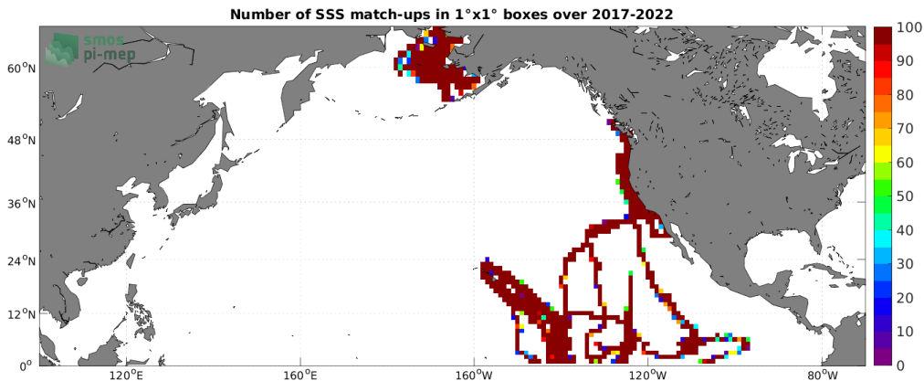
Figure 4: Number of SSS match-ups between Saildrone SSS and the SMAP SSS L3 v5.0 - Monthly (JPL) SSS product for the North Pacific Ocean Pi-MEP region over 1^\circ \times 1^\circ boxes and for the full satellite product period.
