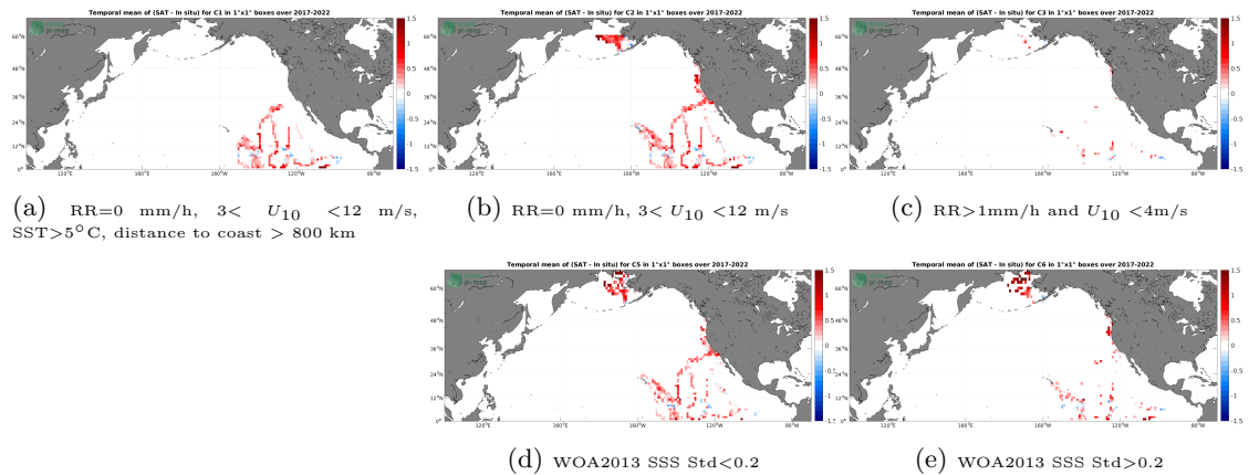
Figure 12: Temporal mean gridded over spatial boxes of size 1^\circ \times 1^\circ of \Delta SSS (SMAP SSS L3 v5.0 - Monthly (JPL) - Saicdrone) for 5 different subdatasets corresponding to:RR=0 mm/h, 3 < U_{10} < 12 m/s, SST > 5^\circ C , distance to coast > 800 km (a), RR=0 mm/h, 3 < U_{10} < 12 m/s (b), RR >1 mm/h and U_{10} < 4 m/s (c), WOA2013 SSS Std <0.2 (d), WOA2013 SSS Std >0.2 (e).
