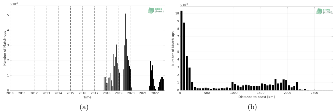
Figure 1: Number of match-ups between Sairdrone and SMAP SSS L3 v5.0 - Monthly (JPL) SSS as a function of time (a) and as function of the distance to coast (b) over the North Pacific Ocean Pi-MEP region and for the full satellite product period.
