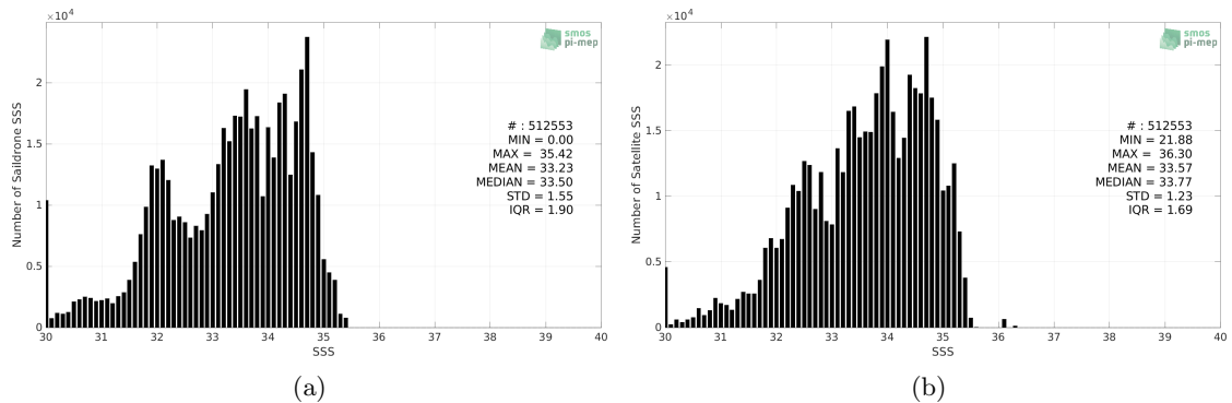
Figure 2: Histograms of SSS from Sairdrone (a) and SMAP SSS L3 v5.0 - Monthly (JPL) (b) considering all match-up pairs per bins of 0.1 over the North Pacific Ocean Pi-MEP region and for the full satellite product period.
