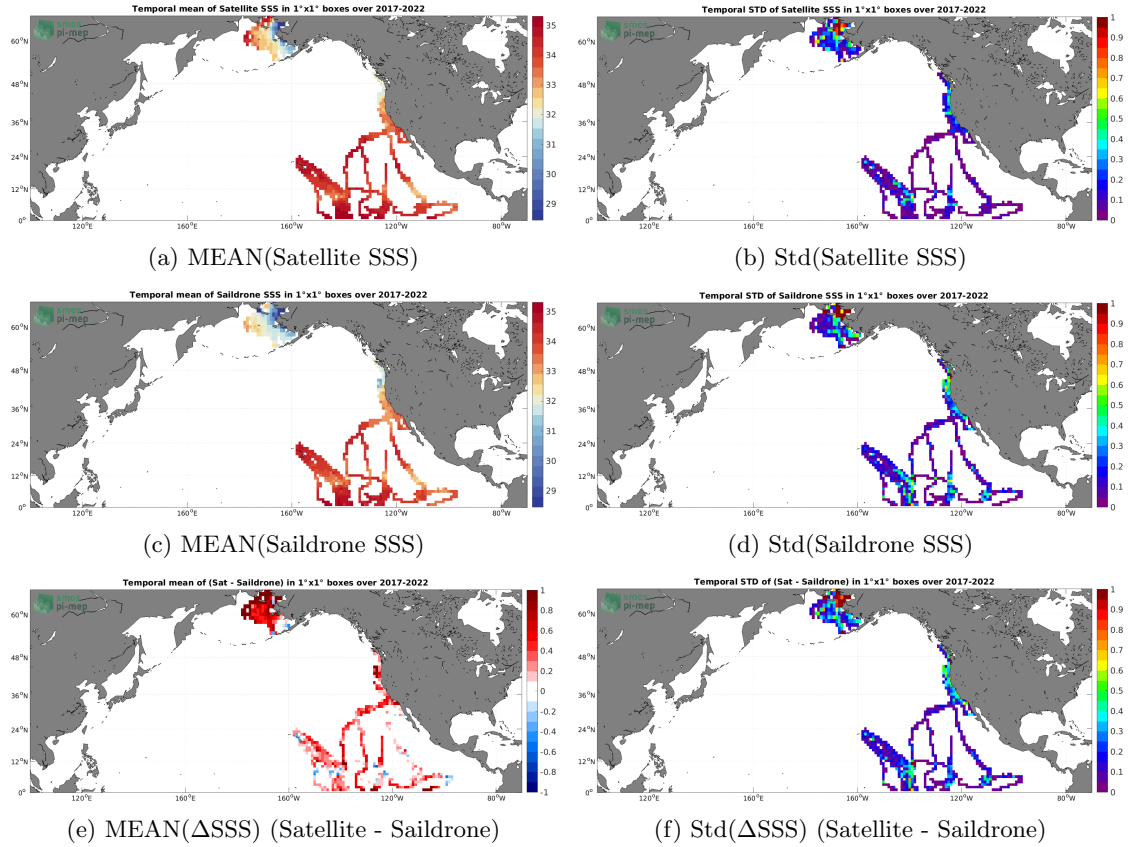
Figure 6: Temporal mean (left) and Std (right) of SSS from SMAP SSS L3 v5.0 - Monthly (JPL) (top), Saildrone (middle), and of \Delta SSS (Satellite - Saildrone). Only match-up pairs are used to generate these maps.
