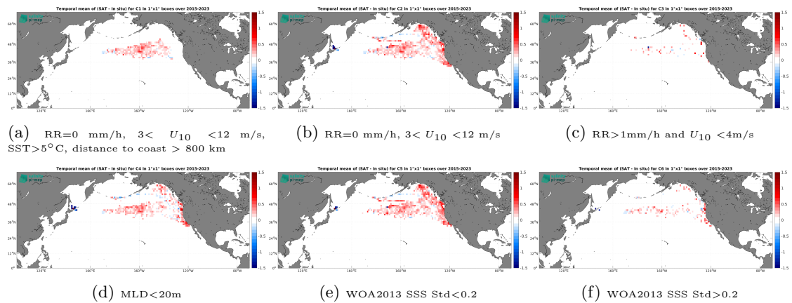
Figure 14: Temporal mean gridded over spatial boxes of size 1^\circ \times 1^\circ of \Delta SSS (SMAP SSS L3 v5.0 - Monthly (JPL) - Marine mammals) for 6 different subdatasets corresponding to:RR=0 mm/h, 3 < U_{10} < 12 m/s, SST >5^\circ C, distance to coast > 800 km (a), RR=0 mm/h, 3 < U_{10} < 12 m/s (b), RR >1 mm/h and U_{10} < 4 m/s (c),MLD <20 m (d),WOA2013 SSS Std <0.2 (e),WOA2013 SSS Std >0.2 (f).
