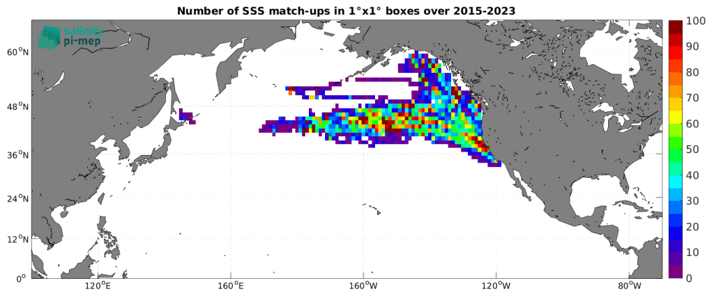
Figure 5: Number of SSS match-ups between Marine mammals SSS and the SMAP SSS L3 v5.0 - Monthly (JPL) SSS product for the North Pacific Ocean Pi-MEP region over 1^\circ \times 1^\circ boxes and for the full satellite product period.
