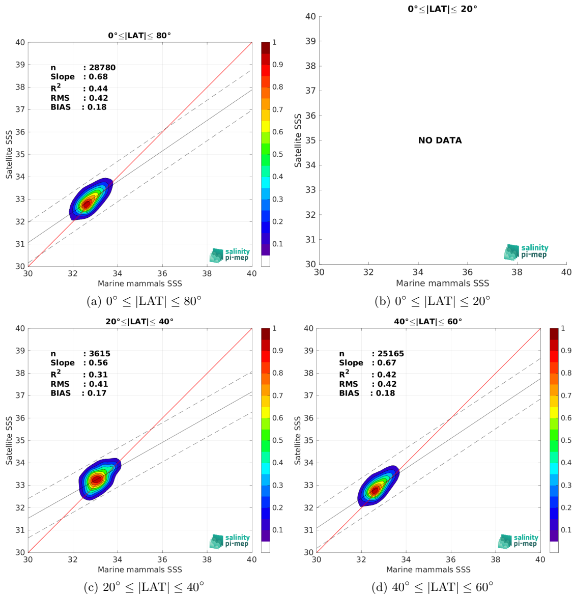
Figure 10: Contour maps of the concentration of SMAP SSS L3 v5.0 - Monthly (JPL) SSS (y-axis) versus Marine mammals SSS (x-axis) at match-up pairs for different latitude bands. For each plot, the red line shows x=y . The black thin and dashed lines indicate a linear fit through the data cloud and the \pm 95\% confidence levels, respectively. The number match-up pairs n , the slope and R^2 coefficient of the linear fit, the root mean square (RMS) and the mean bias between satellite and in situ data are indicated for each latitude band in each plots.
