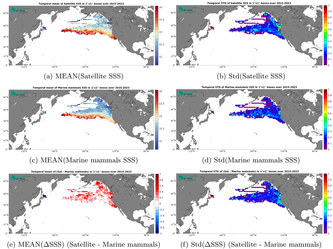
Figure 7: Temporal mean (left) and Std (right) of SSS from SMAP SSS L3 v5.0 - Monthly (JPL) (top), Marine mammals (middle), and of \Delta SSS (Satellite - Marine mammals). Only match-up pairs are used to generate these maps.
