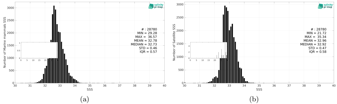
Figure 3: Histograms of SSS from Marine mammals (a) and SMAP SSS L3 v5.0 - Monthly (JPL) (b) considering all match-up pairs per bins of 0.1 over the North Pacific Ocean Pi-MEP region and for the full satellite product period.
