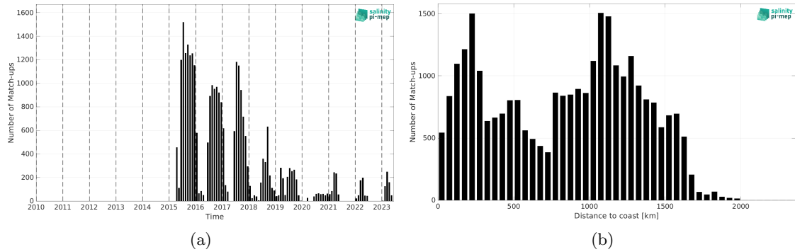
Figure 2: Number of match-ups between Marine mammals and SMAP SSS L3 v5.0 - Monthly (JPL) SSS as a function of time (a) and as function of the distance to coast (b) over the North Pacific Ocean Pi-MEP region and for the full satellite product period.
