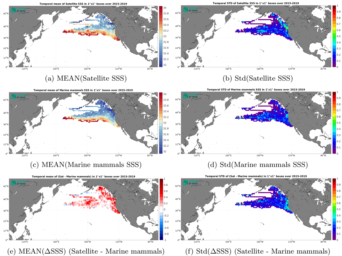
Figure 6: Temporal mean (left) and Std (right) of SSS from SMAP SSS L3 v5.0 - Monthly (JPL) (top), Marine mammals (middle), and of \Delta SSS (Satellite - Marine mammals). Only match-up pairs are used to generate these maps.
