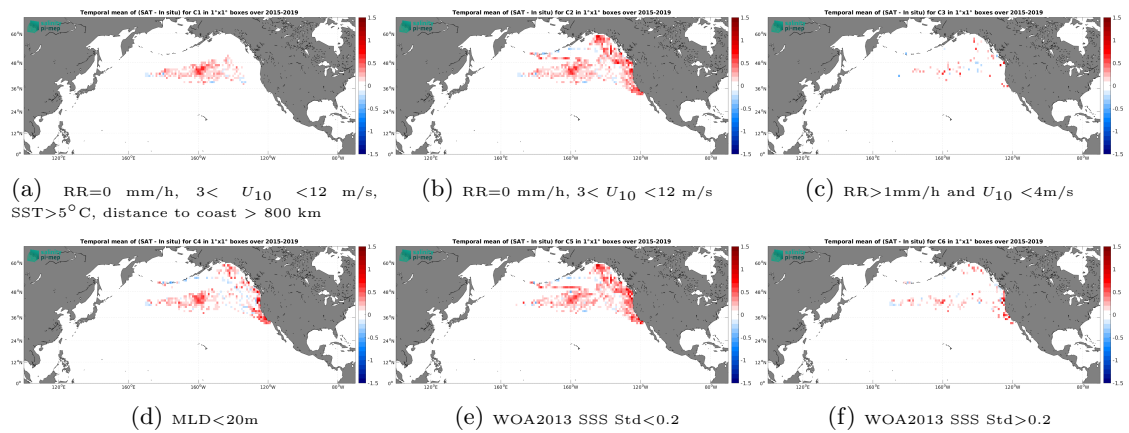
Figure 12: Temporal mean gridded over spatial boxes of size 1^\circ \times 1^\circ of \Delta SSS (SMAP SSS L3 v5.0 - Monthly (JPL) - Marine mammals) for 6 different subdatasets corresponding to:RR=0 mm/h, 3 < U_{10} < 12 m/s, SST > 5^\circ C , distance to coast > 800 km (a), RR=0 mm/h, 3 < U_{10} < 12 m/s (b), RR>1mm/h and U_{10} < 4 m/s (c),MLD<20m (d),WOA2013 SSS Std<0.2 (e),WOA2013 SSS Std>0.2 (f).
