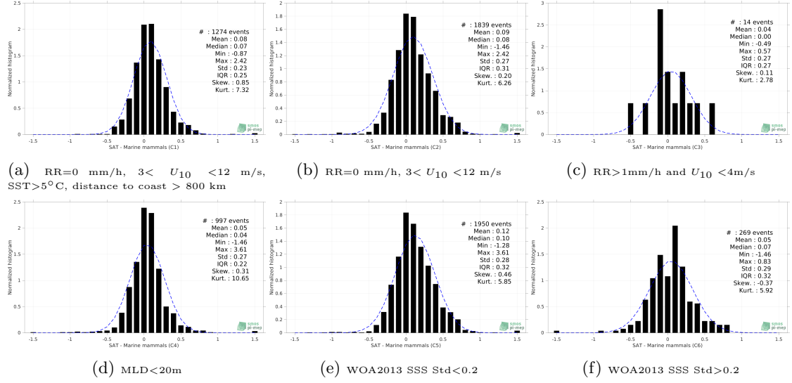
Figure 13: Normalized histogram of \Delta SSS (SMAP SSS L3 v5.0 - Monthly (JPL) - Marine mammals) for 6 different subdatasets corresponding to: RR=0 mm/h, 3 < U_{10} < 12 m/s, SST > 5°C, distance to coast > 800 km (a), RR=0 mm/h, 3 < U_{10} < 12 m/s (b), RR > 1mm/h and U_{10} < 4 m/s (c), MLD < 20m (d), WOA2013 SSS Std < 0.2 (e), WOA2013 SSS Std > 0.2 (f).
