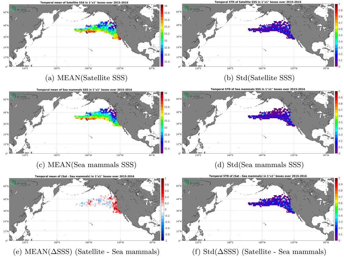
Figure 6: Temporal mean (left) and Std (right) of SSS from SMAP SSS L3 v5.0 - Monthly (JPL) (top), Sea mammals (middle), and of \Delta\text{SSS} (Satellite - Sea mammals). Only match-up pairs are used to generate these maps.
