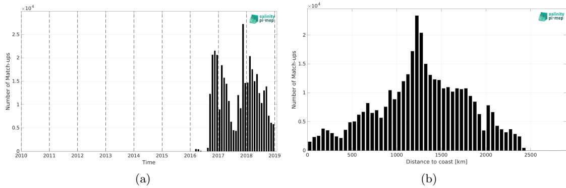
Figure 2: Number of match-ups between Surface drifters and SMAP SSS L3 v5.0 - Monthly (JPL) SSS as a function of time (a) and as function of the distance to coast (b) over the North Pacific Ocean Pi-MEP region and for the full satellite product period.
