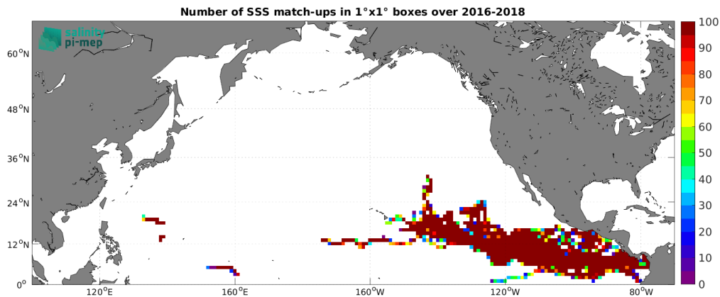
Figure 4: Number of SSS match-ups between Surface drifters SSS and the SMAP SSS L3 v5.0 - Monthly (JPL) SSS product for the North Pacific Ocean Pi-MEP region over 1^\circ \times 1^\circ boxes and for the full satellite product period.
