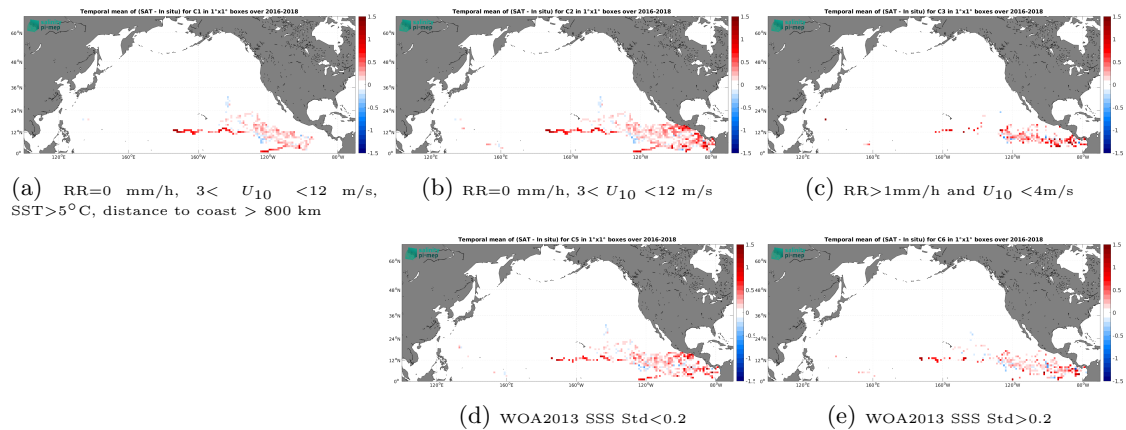
Figure 13: Temporal mean gridded over spatial boxes of size 1^\circ \times 1^\circ of \Delta SSS (SMAP SSS L3 v5.0 - Monthly (JPL) - Surface drifters) for 5 different subdatasets corresponding to:RR=0 mm/h, 3 < U_{10} < 12 m/s, SST >5^\circ\text{C} , distance to coast > 800 km (a), RR=0 mm/h, 3 < U_{10} < 12 m/s (b), RR >1 mm/h and U_{10} < 4 m/s (c), WOA2013 SSS Std <0.2 (d), WOA2013 SSS Std >0.2 (e).
