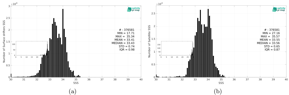
Figure 3: Histograms of SSS from Surface drifters (a) and SMAP SSS L3 v5.0 - Monthly (JPL) (b) considering all match-up pairs per bins of 0.1 over the North Pacific Ocean Pi-MEP region and for the full satellite product period.
