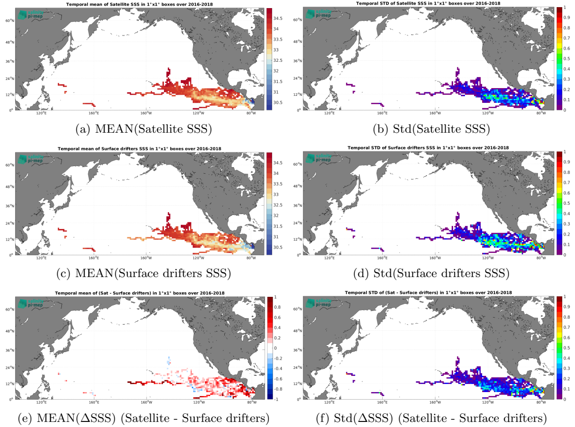
Figure 6: Temporal mean (left) and Std (right) of SSS from SMAP SSS L3 v5.0 - Monthly (JPL) (top), Surface drifters (middle), and of \Delta SSS (Satellite - Surface drifters). Only match-up pairs are used to generate these maps.
