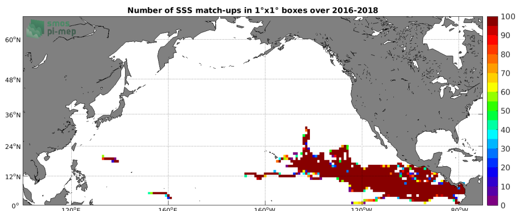
Figure 3: Number of SSS match-ups between Surface drifters SSS and the SMAP SSS L3 v5.0 - Monthly (JPL) SSS product for the North Pacific Ocean Pi-MEP region over 1°x1° boxes and for the full satellite product period.
