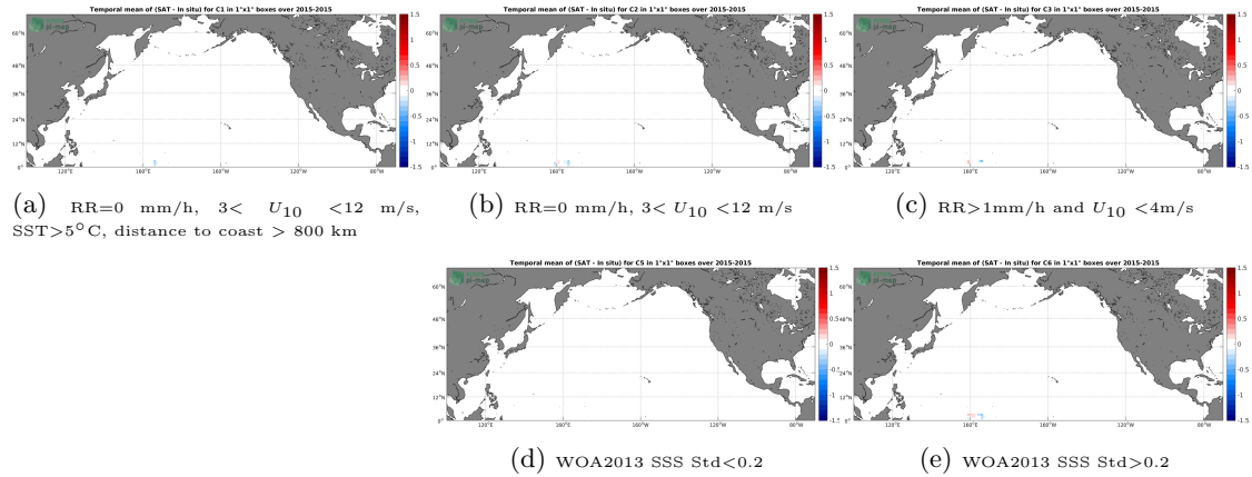
Figure 12: Temporal mean gridded over spatial boxes of size 1^{\circ}\times 1^{\circ} of \Delta SSS (SMAP-L3-JPL-V4.3-8DAY-RUNNING-60KM - TSG-GOSUD-Research-vessel) for 5 different subdatasets corresponding to:RR=0 mm/h, 3 < U_{10} < 12 m/s, SST >5^{\circ}\text{C} , distance to coast > 800 km (a), RR=0 mm/h, 3 < U_{10} < 12 m/s (b), RR >1 mm/h and U_{10} < 4 m/s (c), WOA2013 SSS Std <0.2 (d), WOA2013 SSS Std >0.2 (e).
