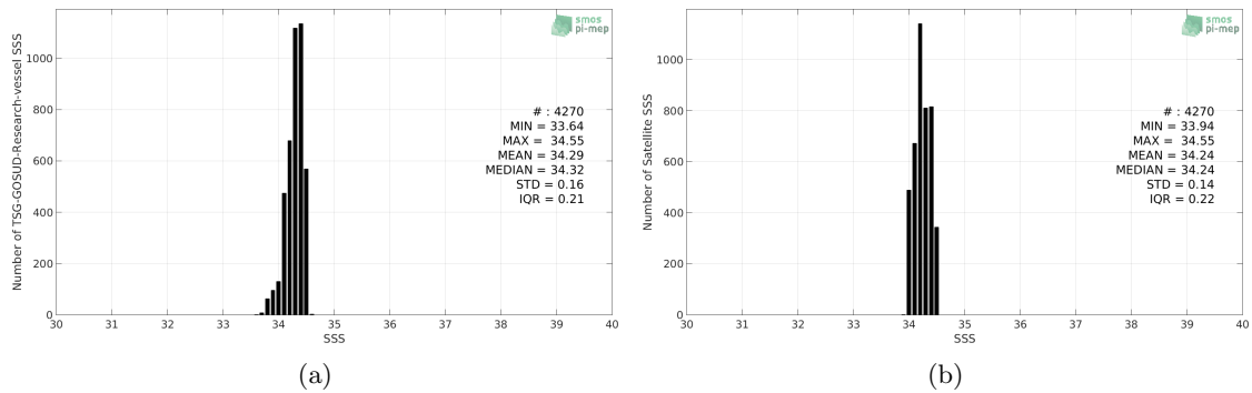
Figure 2: Histograms of SSS from TSG-GOSUD-Research-vessel (a) and SMAP-L3-JPL-V4.3-8DAY-RUNNING-60KM (b) considering all match-up pairs per bins of 0.1 over the North Pacific Ocean Pi-MEP region and for the full satellite product period.
