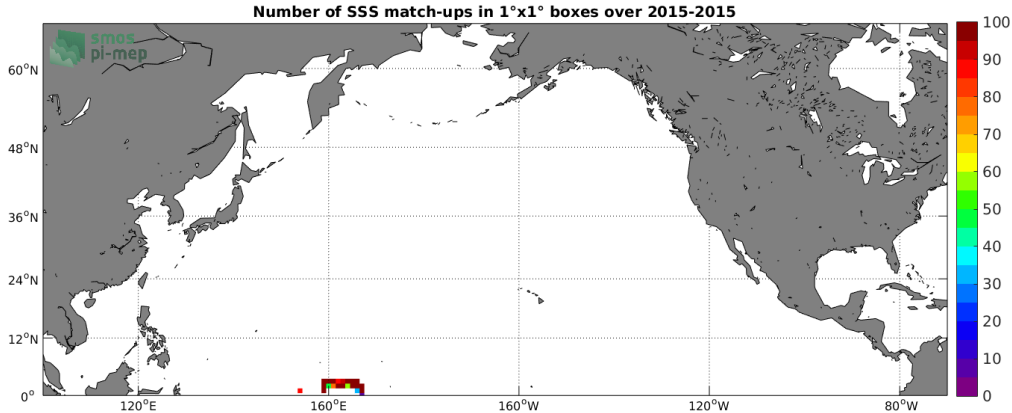
Figure 4: Number of SSS match-ups between TSG-GOSUD-Research-vessel SSS and the SMAP-L3-JPL-V4.3-8DAY-RUNNING-60KM SSS product for the North Pacific Ocean Pi-MEP region over 1^\circ \times 1^\circ boxes and for the full satellite product period.
