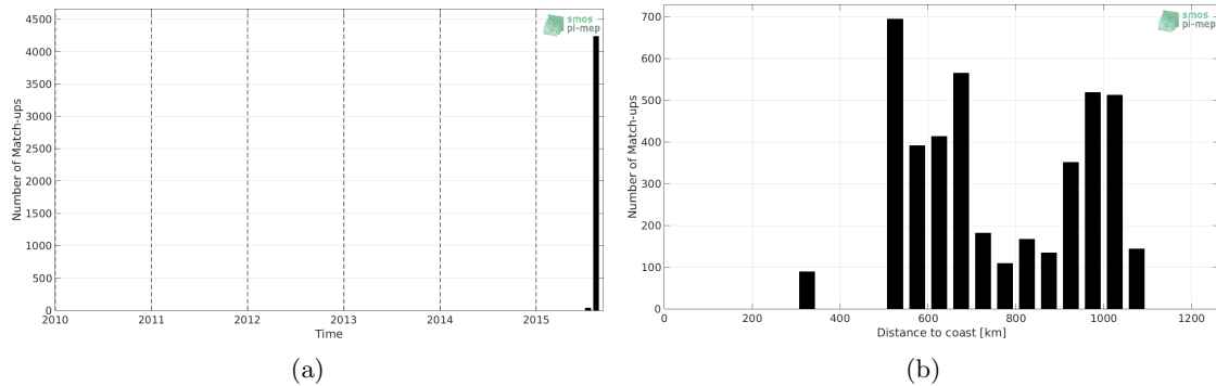
Figure 1: Number of match-ups between TSG-GOSUD-Research-vessel and SMAP-L3-JPL-V4.3-8DAY-RUNNING-60KM SSS as a function of time (a) and as function of the distance to coast (b) over the North Pacific Ocean Pi-MEP region and for the full satellite product period.
