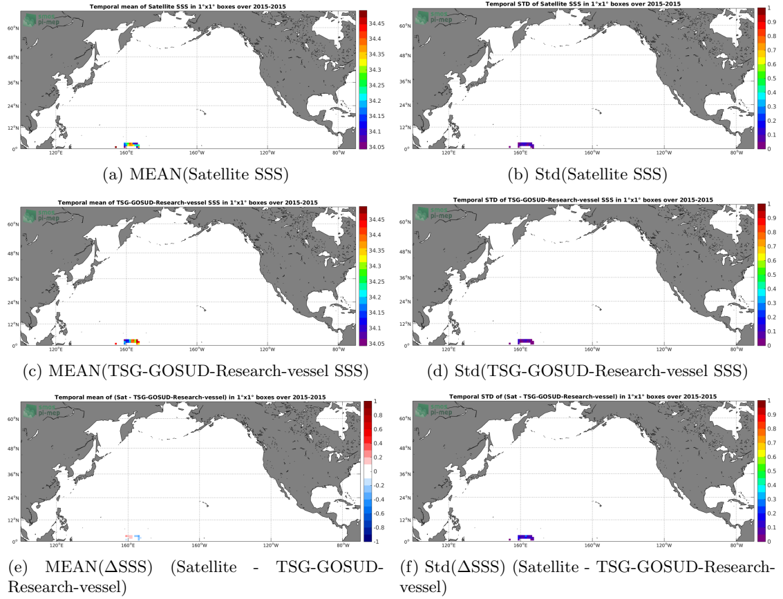
Figure 6: Temporal mean (left) and Std (right) of SSS from SMAP-L3-JPL-V4.3-8DAY-RUNNING-60KM (top), TSG-GOSUD-Research-vessel (middle), and of \Delta SSS (Satellite - TSG-GOSUD-Research-vessel). Only match-up pairs are used to generate these maps.
