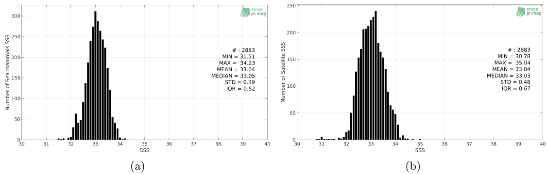
Figure 2: Histograms of SSS from Sea mammals (a) and SMAP-L3-JPL-V4.3-8DAY-RUNNING-60KM (b) considering all match-up pairs per bins of 0.1 over the North Pacific Ocean Pi-MEP region and for the full satellite product period.
