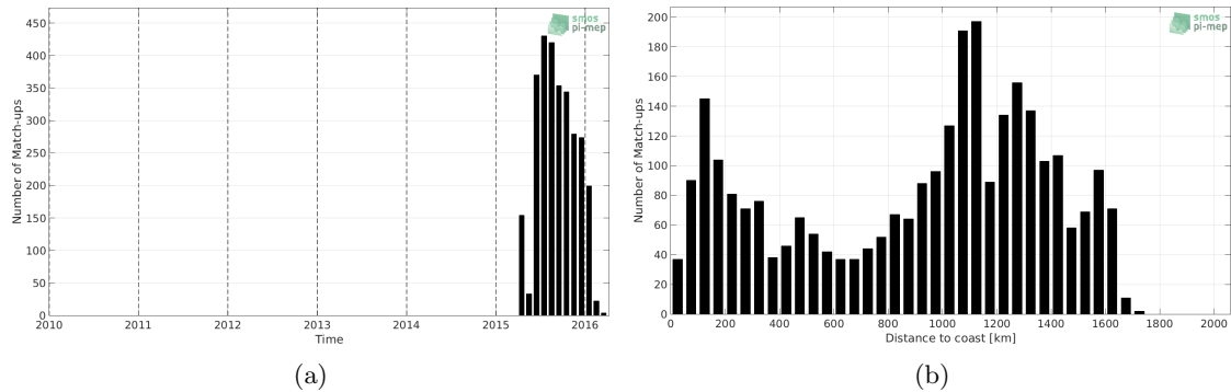
Figure 1: Number of match-ups between Sea mammals and SMAP-L3-JPL-V4.3-8DAY-RUNNING-60KM SSS as a function of time (a) and as function of the distance to coast (b) over the North Pacific Ocean Pi-MEP region and for the full satellite product period.
