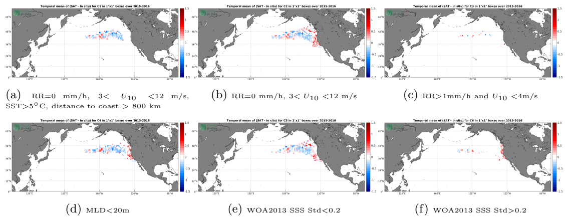
Figure 12: Temporal mean gridded over spatial boxes of size 1^\circ \times 1^\circ of \Delta SSS (SMAP-L3-JPL-V4.3-8DAY-RUNNING-60KM - Sea mammals) for 6 different subdatasets corresponding to:RR=0 mm/h, 3 < U_{10} < 12 m/s, SST >5^\circ C, distance to coast > 800 km (a), RR=0 mm/h, 3 < U_{10} < 12 m/s (b), RR >1 mm/h and U_{10} < 4 m/s (c),MLD <20 m (d),WOA2013 SSS Std <0.2 (e),WOA2013 SSS Std >0.2 (f).
