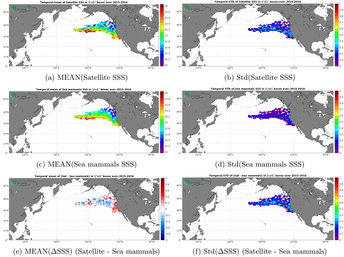
Figure 6: Temporal mean (left) and Std (right) of SSS from SMAP-L3-JPL-V4.3-8DAY-RUNNING-60KM (top), Sea mammals (middle), and of \Delta SSS (Satellite - Sea mammals). Only match-up pairs are used to generate these maps.
