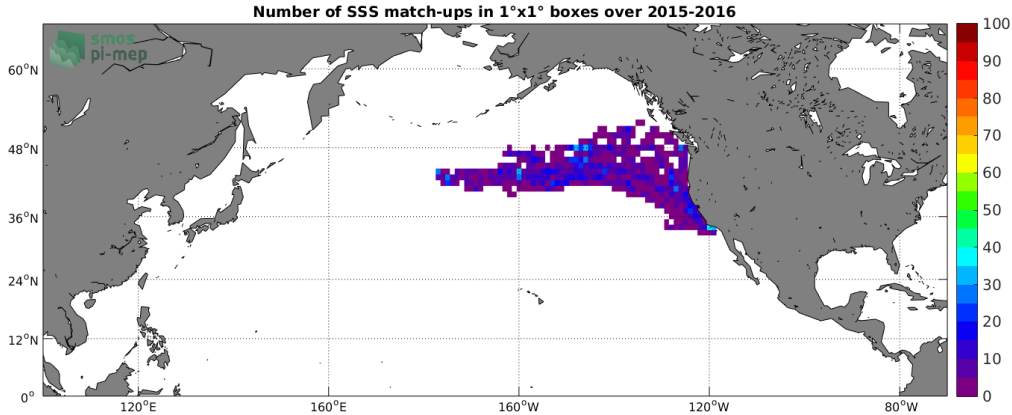
Figure 4: Number of SSS match-ups between Sea mammals SSS and the SMAP-L3-JPL-V4.3-8DAY-RUNNING-60KM SSS product for the North Pacific Ocean Pi-MEP region over 1^\circ \times 1^\circ boxes and for the full satellite product period.
