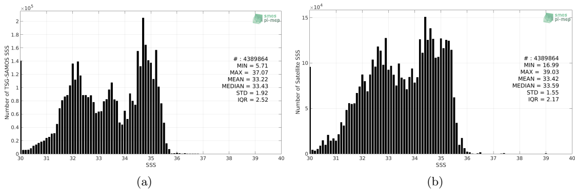
Figure 2: Histograms of SSS from TSG-SAMOS (a) and SMAP-L3-JPL-V4.3-MONTHLY-60KM (b) considering all match-up pairs per bins of 0.1 over the North Pacific Ocean Pi-MEP region and for the full satellite product period.
