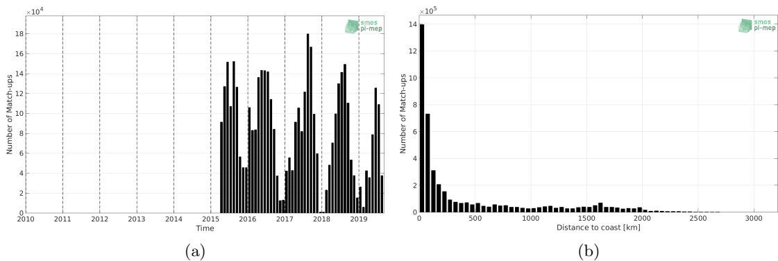
Figure 1: Number of match-ups between TSG-SAMOS and SMAP-L3-JPL-V4.3-MONTHLY-60KM SSS as a function of time (a) and as function of the distance to coast (b) over the North Pacific Ocean Pi-MEP region and for the full satellite product period.
