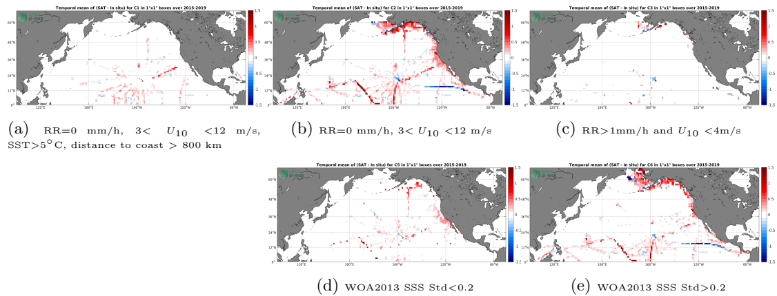
Figure 12: Temporal mean gridded over spatial boxes of size 1^\circ \times 1^\circ of \Delta SSS (SMAP-L3-JPL-V4.3-MONTHLY-60KM - TSG-SAMOS) for 5 different subdatasets corresponding to:RR=0 mm/h, 3 < U_{10} < 12 m/s, SST >5^\circ\text{C} , distance to coast > 800 km (a), RR=0 mm/h, 3 < U_{10} < 12 m/s (b), RR >1 mm/h and U_{10} < 4 m/s (c), WOA2013 SSS Std <0.2 (d), WOA2013 SSS Std >0.2 (e).
