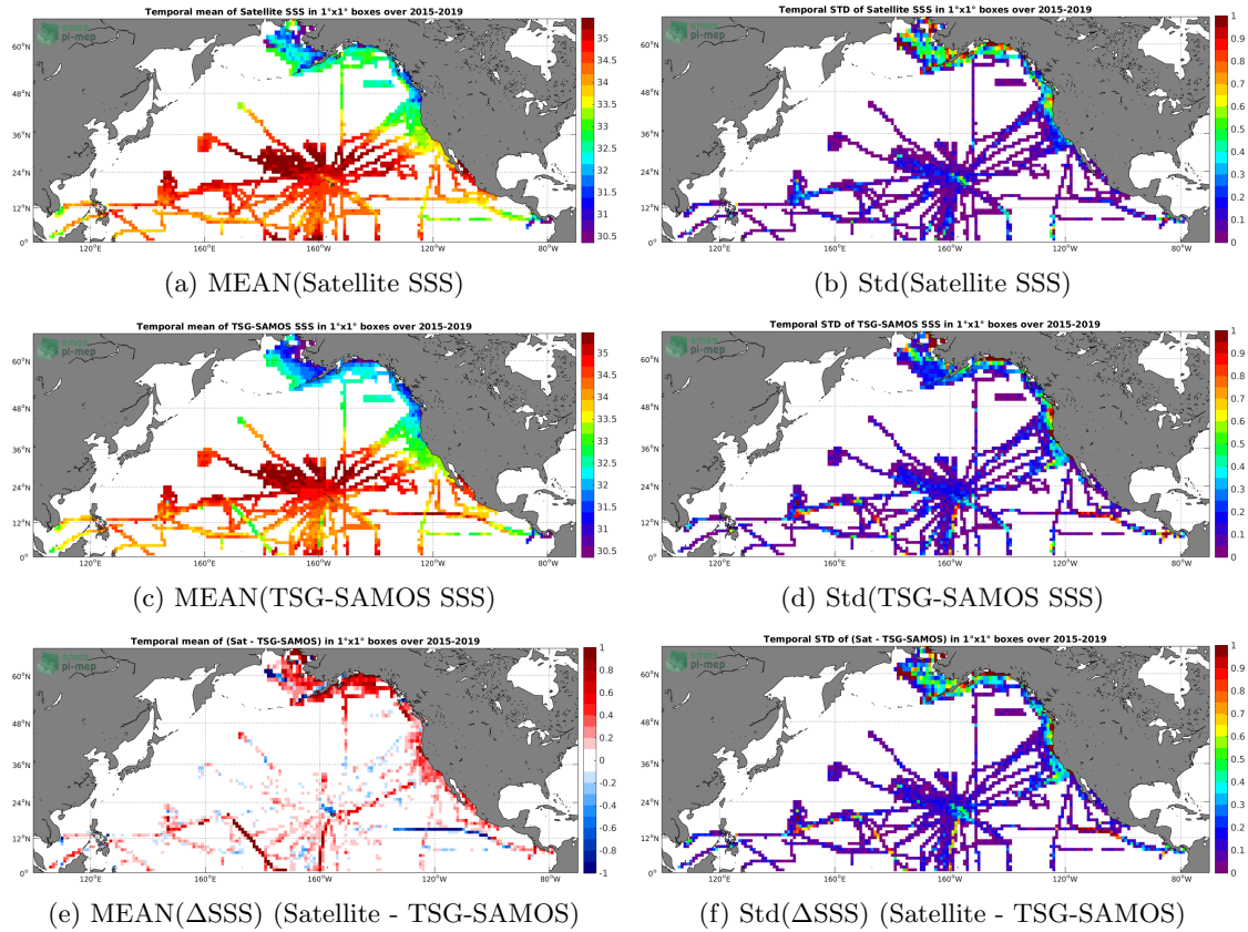
Figure 6: Temporal mean (left) and Std (right) of SSS from SMAP-L3-JPL-V4.3-MONTHLY-60KM (top), TSG-SAMOS (middle), and of \Delta SSS (Satellite - TSG-SAMOS). Only match-up pairs are used to generate these maps.
