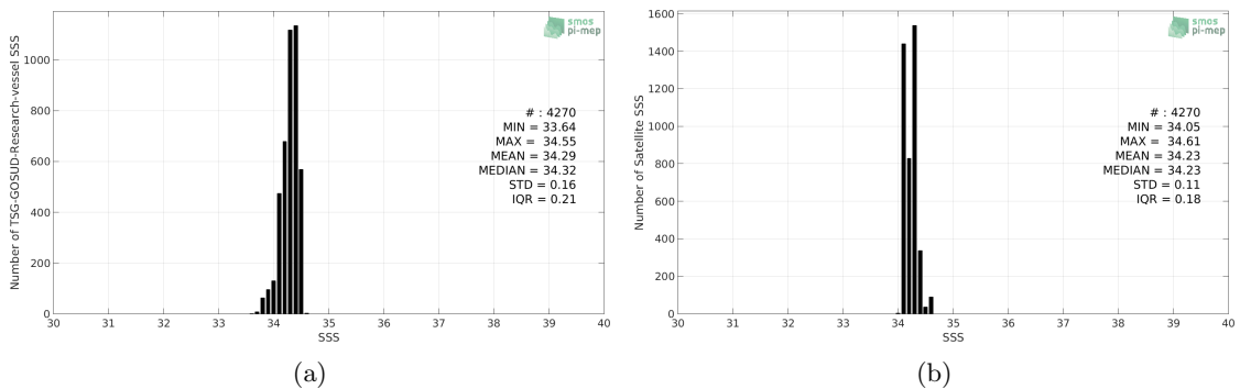
Figure 2: Histograms of SSS from TSG-GOSUD-Research-vessel (a) and SMAP-L3-JPL-V4.3-MONTHLY-60KM (b) considering all match-up pairs per bins of 0.1 over the North Pacific Ocean Pi-MEP region and for the full satellite product period.
