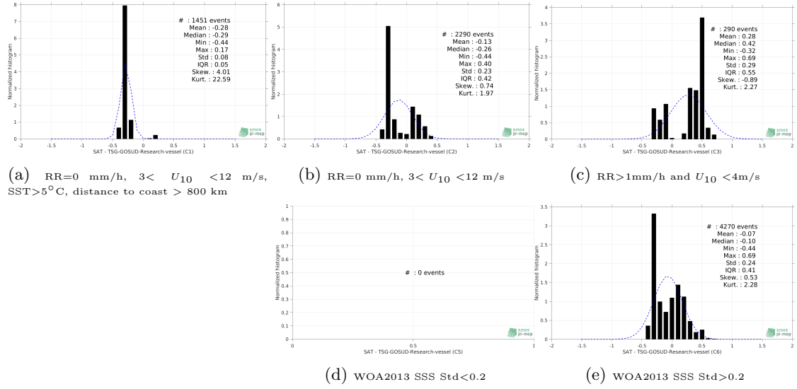
Figure 13: Normalized histogram of \Delta\text{SSS} (SMAP-L3-JPL-V4.3-MONTHLY-60KM - TSG-GOSUD-Research-vessel) for 5 different subdatasets corresponding to: RR=0 mm/h, 3 < U_{10} < 12 m/s, SST > 5^\circ\text{C} , distance to coast > 800 km (a), RR=0 mm/h, 3 < U_{10} < 12 m/s (b), RR > 1 mm/h and U_{10} < 4 m/s (c), WOA2013 SSS Std <0.2 (d), WOA2013 SSS Std >0.2 (e).
