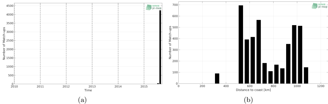
Figure 1: Number of match-ups between TSG-GOSUD-Research-vessel and SMAP-L3-JPL-V4.3-MONTHLY-60KM SSS as a function of time (a) and as function of the distance to coast (b) over the North Pacific Ocean Pi-MEP region and for the full satellite product period.
