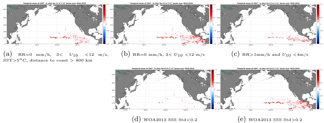
Figure 11: Temporal mean gridded over spatial boxes of size 1^\circ \times 1^\circ of \Delta SSS (SMAP-L3-JPL-V4.3-MONTHLY-60KM - Surface drifters) for 5 different subdatasets corresponding to:RR=0 mm/h, 3 < U_{10} < 12 m/s, SST > 5^\circ C , distance to coast > 800 km (a), RR=0 mm/h, 3 < U_{10} < 12 m/s (b), RR >1 mm/h and U_{10} < 4 m/s (c), WOA2013 SSS Std <0.2 (d), WOA2013 SSS Std >0.2 (e).
