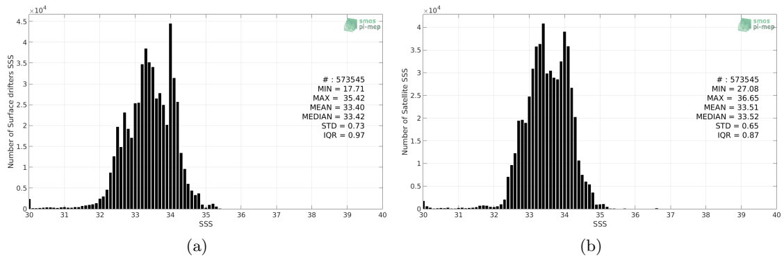
Figure 2: Histograms of SSS from Surface drifters (a) and SMAP-L3-JPL-V4.3-MONTHLY-60KM (b) considering all match-up pairs per bins of 0.1 over the North Pacific Ocean Pi-MEP region and for the full satellite product period.
