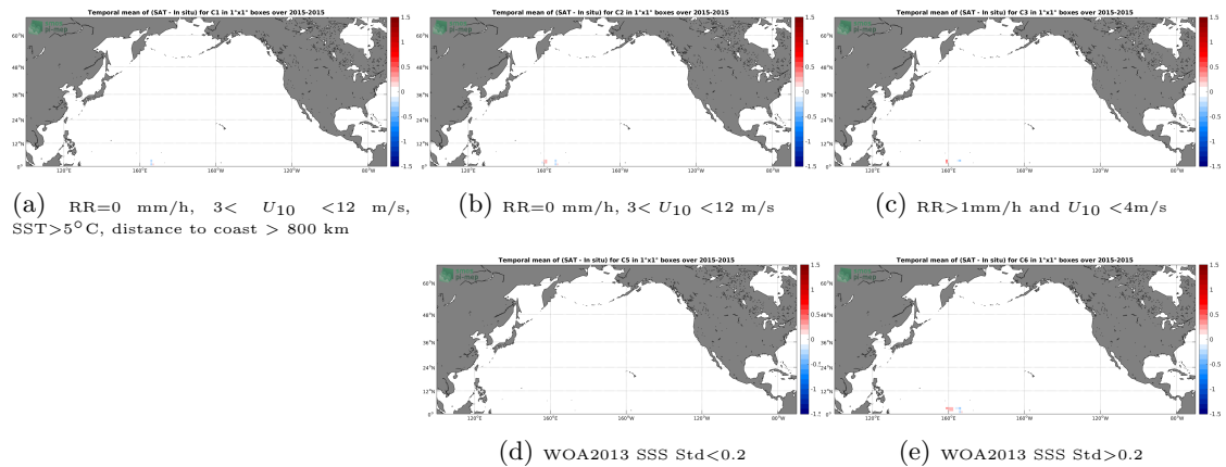
Figure 12: Temporal mean gridded over spatial boxes of size 1^\circ \times 1^\circ of \Delta SSS (SMAP-L3-JPL-V4.2-8DAY-RUNNING-60KM - TSG-GOSUD-Research-vessel) for 5 different subdatasets corresponding to:RR=0 mm/h, 3 < U_{10} < 12 m/s, SST >5^\circ C, distance to coast > 800 km (a), RR=0 mm/h, 3 < U_{10} < 12 m/s (b), RR >1 mm/h and U_{10} < 4 m/s (c), WOA2013 SSS Std <0.2 (d), WOA2013 SSS Std >0.2 (e).
