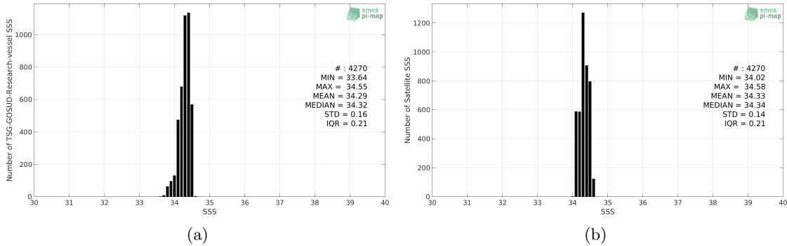
Figure 2: Histograms of SSS from TSG-GOSUD-Research-vessel (a) and SMAP-L3-JPL-V4.2-8DAY-RUNNING-60KM (b) considering all match-up pairs per bins of 0.1 over the North Pacific Ocean Pi-MEP region and for the full satellite product period.
