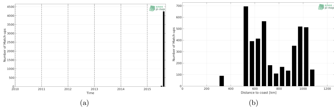
Figure 1: Number of match-ups between TSG-GOSUD-Research-vessel and SMAP-L3-JPL-V4.2-8DAY-RUNNING-60KM SSS as a function of time (a) and as function of the distance to coast (b) over the North Pacific Ocean Pi-MEP region and for the full satellite product period.
