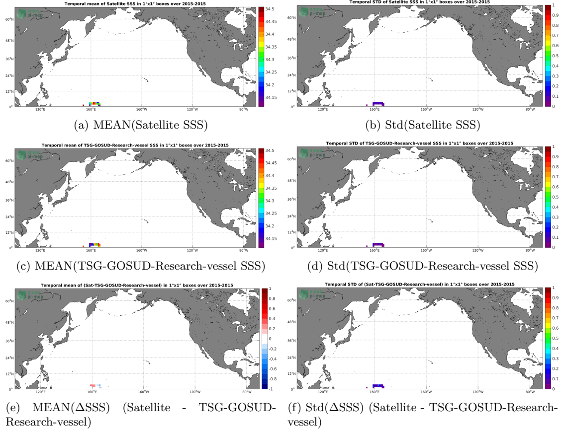
Figure 6: Temporal mean (left) and Std (right) of SSS from SMAP-L3-JPL-V4.2-8DAY-RUNNING-60KM (top), TSG-GOSUD-Research-vessel (middle), and of \Delta SSS (Satellite - TSG-GOSUD-Research-vessel). Only match-up pairs are used to generate these maps.
