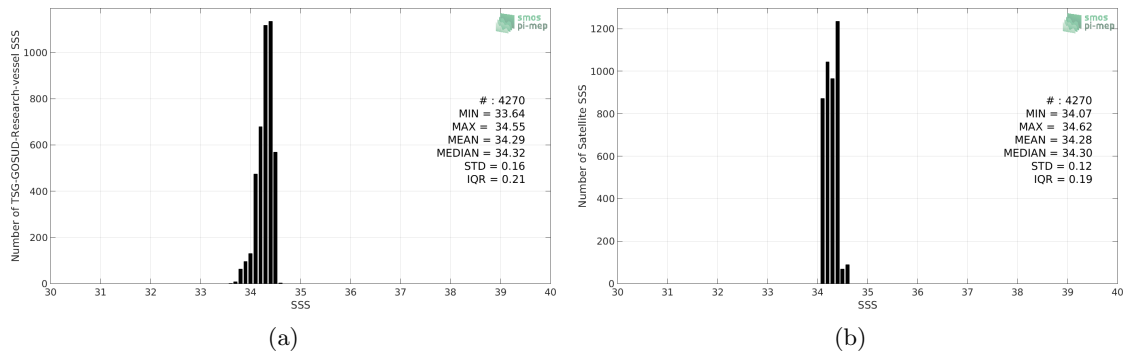
Figure 2: Histograms of SSS from TSG-GOSUD-Research-vessel (a) and SMAP-L3-JPL-V4.2-MONTHLY-60KM (b) considering all match-up pairs per bins of 0.1 over the North Pacific Ocean Pi-MEP region and for the full satellite product period.
