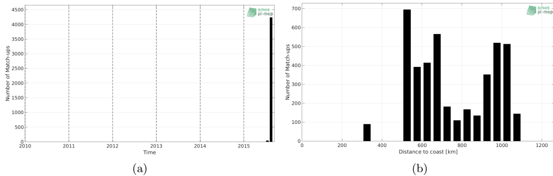
Figure 1: Number of match-ups between TSG-GOSUD-Research-vessel and SMAP-L3-JPL-V4.2-MONTHLY-60KM SSS as a function of time (a) and as function of the distance to coast (b) over the North Pacific Ocean Pi-MEP region and for the full satellite product period.
