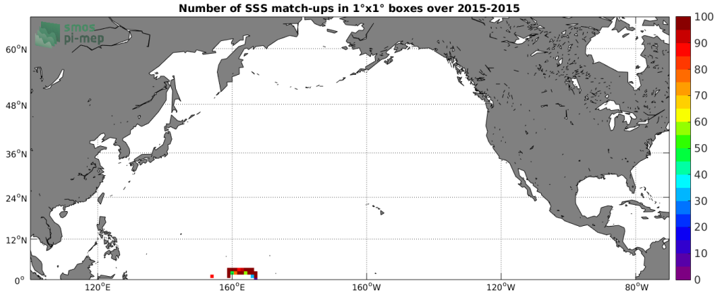
Figure 4: Number of SSS match-ups between TSG-GOSUD-Research-vessel SSS and the SMAP-L3-JPL-V4.2-MONTHLY-60KM SSS product for the North Pacific Ocean Pi-MEP region over 1^\circ \times 1^\circ boxes and for the full satellite product period.
