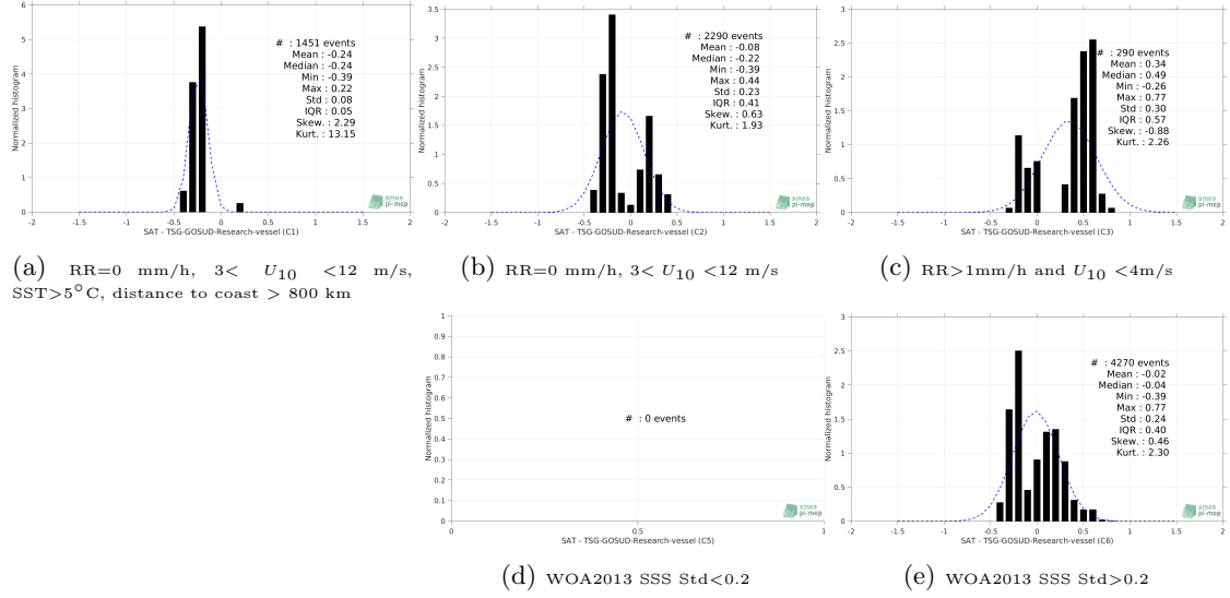
Figure 13: Normalized histogram of \Delta\text{SSS} (SMAP-L3-JPL-V4.2-MONTHLY-60KM - TSG-GOSUD-Research-vessel) for 5 different subdatasets corresponding to: RR=0 mm/h, 3 < U_{10} < 12 m/s, SST > 5^{\circ}\text{C} , distance to coast > 800 km (a), RR=0 mm/h, 3 < U_{10} < 12 m/s (b), RR > 1\text{mm/h} and U_{10} < 4\text{m/s} (c), WOA2013 SSS \text{Std} < 0.2 (d), WOA2013 SSS \text{Std} > 0.2 (e).
