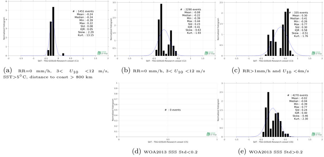
Figure 13: Normalized histogram of \Delta SSS (SMAP-L3-JPL-V4.2-MONTHLY-60KM - TSG-GOSUD-Research-vessel) for 5 different subdatasets corresponding to: RR=0 mm/h, 3 < U_{10} < 12 m/s, SST>5°C, distance to coast > 800 km (a), RR=0 mm/h, 3 < U_{10} < 12 m/s (b), RR>1mm/h and U_{10} < 4 m/s (c), WOA2013 SSS Std<0.2 (d), WOA2013 SSS Std>0.2 (e).
