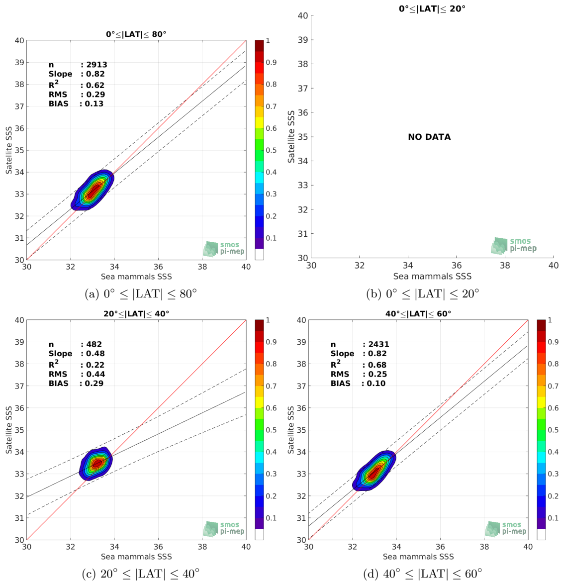
Figure 9: Contour maps of the concentration of SMAP-L3-JPL-V4.2-MONTHLY-60KM SSS (y-axis) versus Sea mammals SSS (x-axis) at match-up pairs for different latitude bands. For each plot, the red line shows x=y . The black thin and dashed lines indicate a linear fit through the data cloud and the \pm 95\% confidence levels, respectively. The number match-up pairs n , the slope and R^2 coefficient of the linear fit, the root mean square (RMS) and the mean bias between satellite and in situ data are indicated for each latitude band in each plots.
