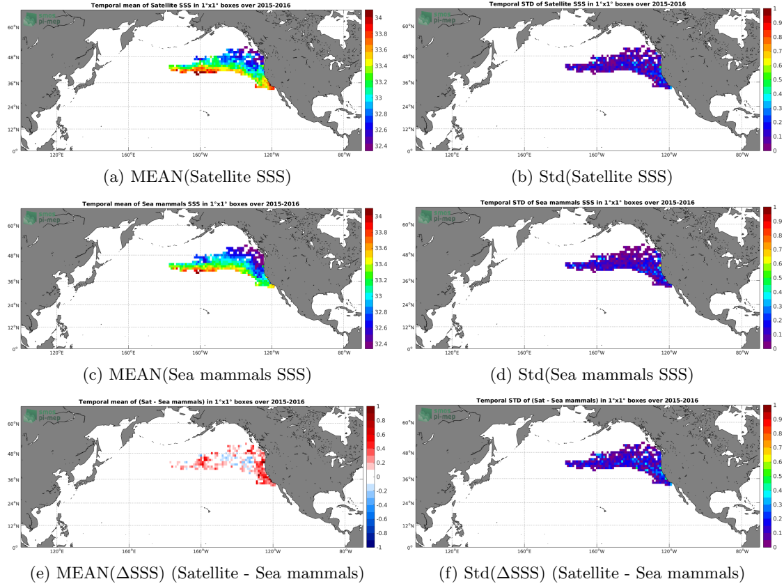
Figure 6: Temporal mean (left) and Std (right) of SSS from SMAP-L3-JPL-V4.2-MONTHLY-60KM (top), Sea mammals (middle), and of \Delta SSS (Satellite - Sea mammals). Only match-up pairs are used to generate these maps.
