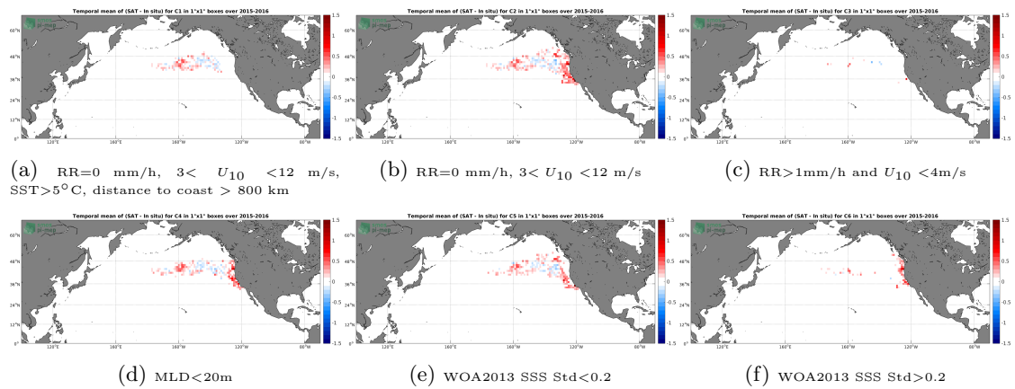
Figure 12: Temporal mean gridded over spatial boxes of size 1^\circ \times 1^\circ of \Delta SSS (SMAP-L3-JPL-V4.2-MONTHLY-60KM - Sea mammals) for 6 different subdatasets corresponding to:RR=0 mm/h, 3 < U_{10} < 12 m/s, SST >5^\circ C, distance to coast > 800 km (a), RR=0 mm/h, 3 < U_{10} < 12 m/s (b), RR >1 mm/h and U_{10} < 4 m/s (c),MLD <20 m (d),WOA2013 SSS Std <0.2 (e),WOA2013 SSS Std >0.2 (f).
