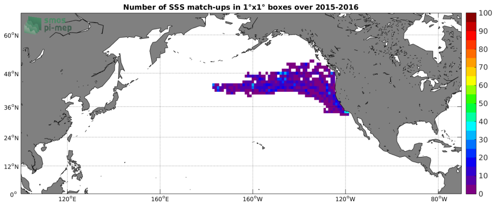
Figure 4: Number of SSS match-ups between Sea mammals SSS and the SMAP-L3-JPL-V4.2-MONTHLY-60KM SSS product for the North Pacific Ocean Pi-MEP region over 1^\circ \times 1^\circ boxes and for the full satellite product period.
