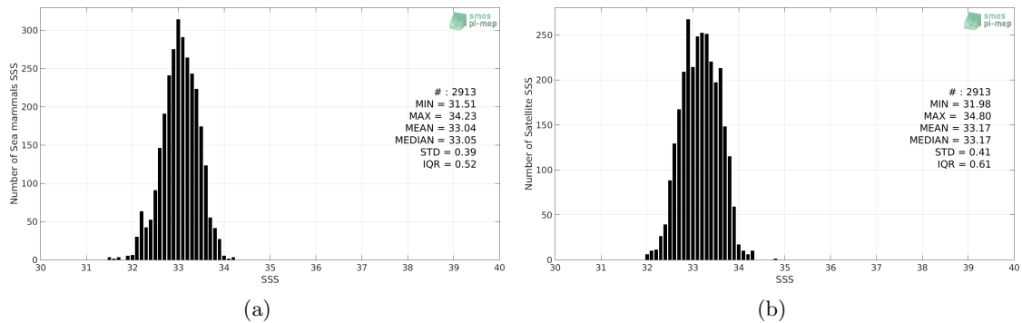
Figure 2: Histograms of SSS from Sea mammals (a) and SMAP-L3-JPL-V4.2-MONTHLY-60KM (b) considering all match-up pairs per bins of 0.1 over the North Pacific Ocean Pi-MEP region and for the full satellite product period.
