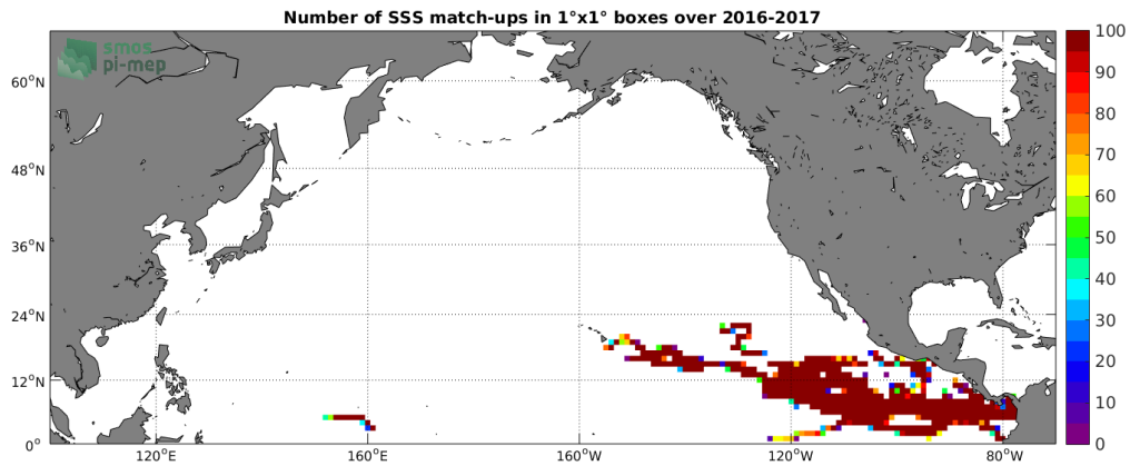
Figure 3: Number of SSS match-ups between Surface drifters SSS and the SMAP-L3-JPL-V4.2-MONTHLY-60KM SSS product for the North Pacific Ocean Pi-MEP region over 1°x1° boxes and for the full satellite product period.
