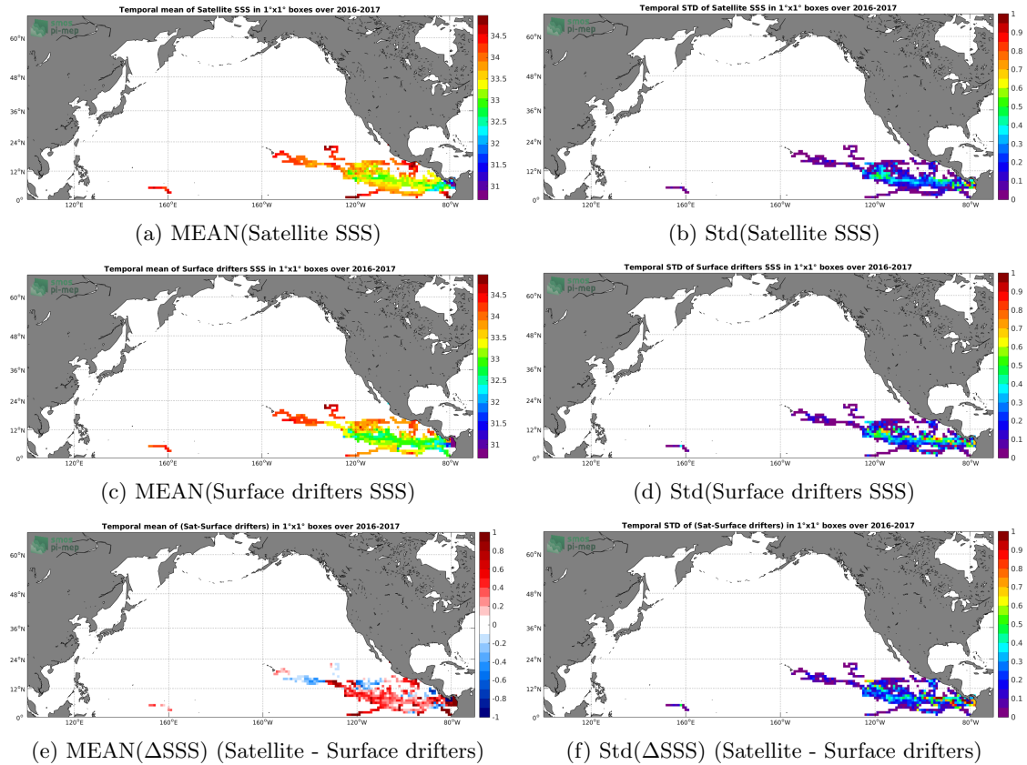
Figure 5: Temporal mean (left) and Std (right) of SSS from SMAP-L3-JPL-V4.2-MONTHLY-60KM (top), Surface drifters (middle), and of \Delta SSS (Satellite - Surface drifters). Only match-up pairs are used to generate these maps.
