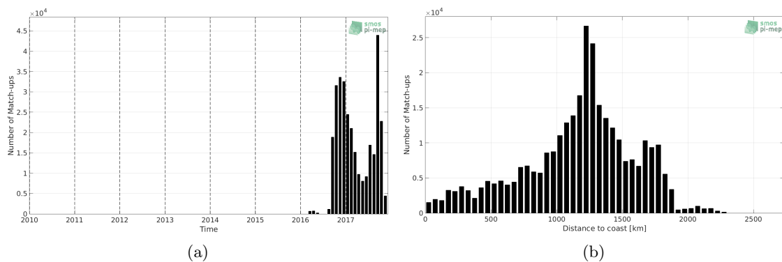
Figure 1: Number of match-ups between Surface drifters and SMAP-L3-JPL-V4.2-MONTHLY-60KM SSS as a function of time (a) and as function of the distance to coast (b) over the North Pacific Ocean Pi-MEP region and for the full satellite product period.
