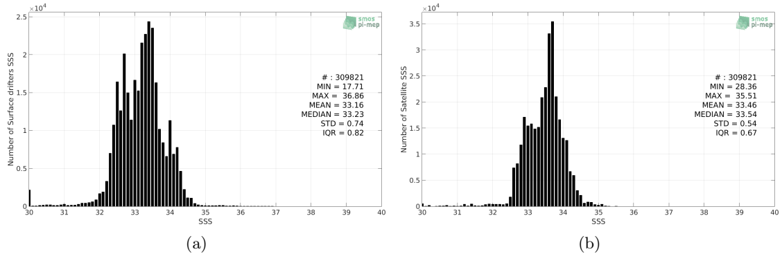
Figure 2: Histograms of SSS from Surface drifters (a) and SMAP-L3-JPL-V4.2-MONTHLY-60KM (b) considering all match-up pairs per bins of 0.1 over the North Pacific Ocean Pi-MEP region and for the full satellite product period.
