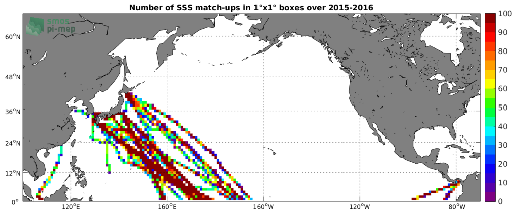
Figure 4: Number of SSS match-ups between TSG-LEGOS-DM SSS and the SMAP-L3-JPL-V4-8DAY-RUNNING-60KM SSS product for the North Pacific Ocean Pi-MEP region over 1^\circ \times 1^\circ boxes and for the full satellite product period.
