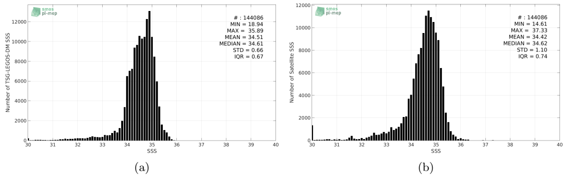
Figure 2: Histograms of SSS from TSG-LEGOS-DM (a) and SMAP-L3-JPL-V4-8DAY-RUNNING-60KM (b) considering all match-up pairs per bins of 0.1 over the North Pacific Ocean Pi-MEP region and for the full satellite product period.
