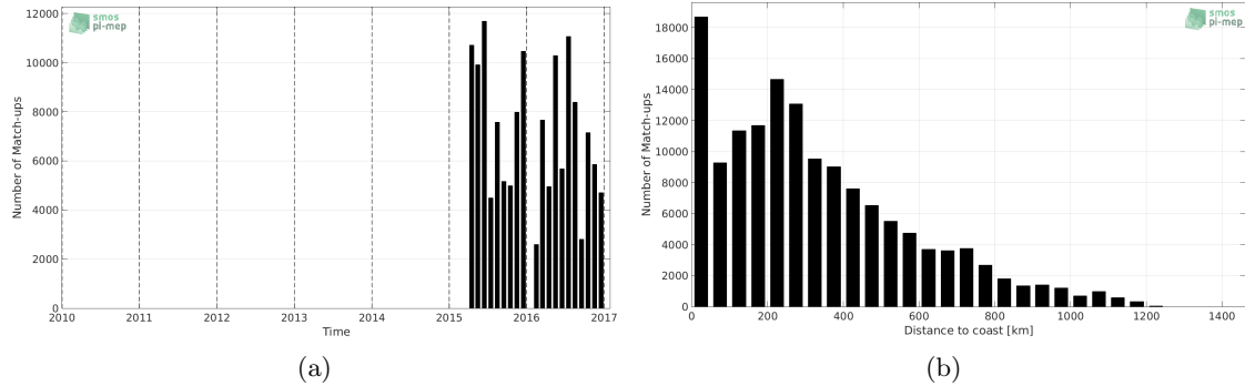
Figure 1: Number of match-ups between TSG-LEGOS-DM and SMAP-L3-JPL-V4-8DAY-RUNNING-60KM SSS as a function of time (a) and as function of the distance to coast (b) over the North Pacific Ocean Pi-MEP region and for the full satellite product period.
