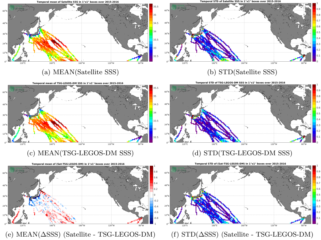
Figure 6: Temporal mean (left) and STD (right) of SSS from SMAP-L3-JPL-V4-8DAY-RUNNING-60KM (top), TSG-LEGOS-DM (middle), and of \Delta SSS (Satellite - TSG-LEGOS-DM). Only match-up pairs are used to generate these maps.
