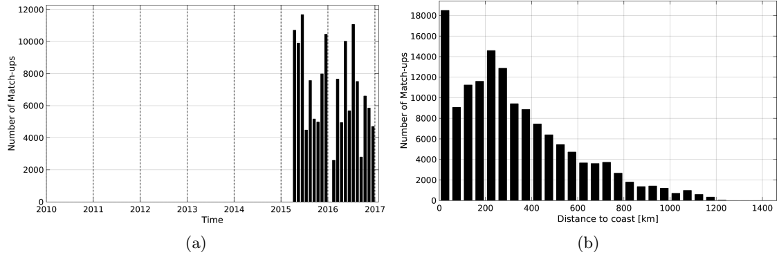
Figure 1: Number of match-ups between TSG-LEGOS-DM and SMAP-L3-JPL-V4-8DAY-RUNNING-60KM SSS as a function of time (a) and as function of the distance to coast (b) over the North Pacific Ocean Pi-MEP region and for the full satellite product period.
