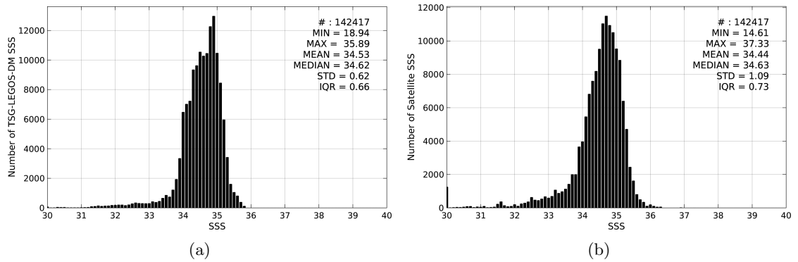
Figure 2: Histograms of SSS from TSG-LEGOS-DM (a) and SMAP-L3-JPL-V4-8DAY-RUNNING-60KM (b) considering all match-up pairs per bins of 0.1 over the North Pacific Ocean Pi-MEP region and for the full satellite product period.
