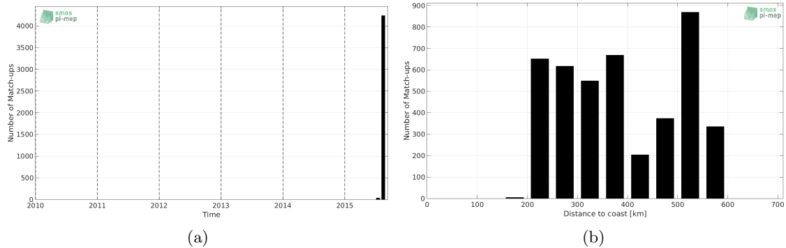
Figure 1: Number of match-ups between TSG-GOSUD-Research-vessel and SMAP-L3-JPL-V4-8DAY-RUNNING-60KM SSS as a function of time (a) and as function of the distance to coast (b) over the North Pacific Ocean Pi-MEP region and for the full satellite product period.
