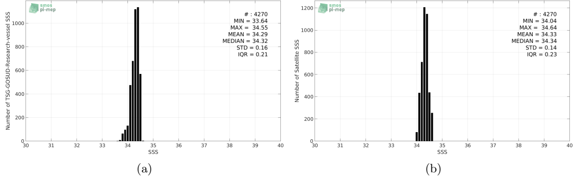
Figure 2: Histograms of SSS from TSG-GOSUD-Research-vessel (a) and SMAP-L3-JPL-V4-8DAY-RUNNING-60KM (b) considering all match-up pairs per bins of 0.1 over the North Pacific Ocean Pi-MEP region and for the full satellite product period.
