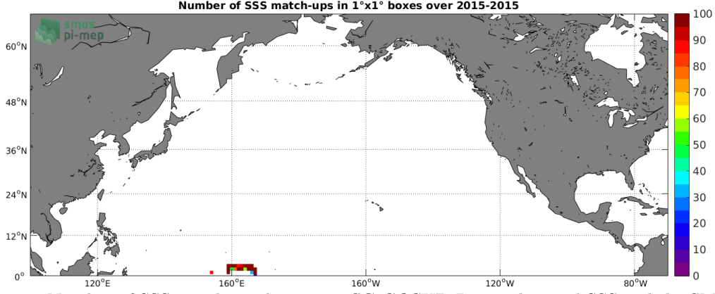
Figure 4: Number of SSS match-ups between TSG-GOSUD-Research-vessel SSS and the SMAP-L3-JPL-V4-8DAY-RUNNING-60KM SSS product for the North Pacific Ocean Pi-MEP region over 1^\circ \times 1^\circ boxes and for the full satellite product period.
