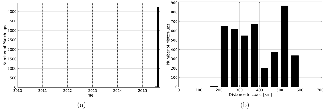
Figure 1: Number of match-ups between TSG-GOSUD-Research-vessel and SMAP-L3-JPL-V4-8DAY-RUNNING-60KM SSS as a function of time (a) and as function of the distance to coast (b) over the North Pacific Ocean Pi-MEP region and for the full satellite product period.
