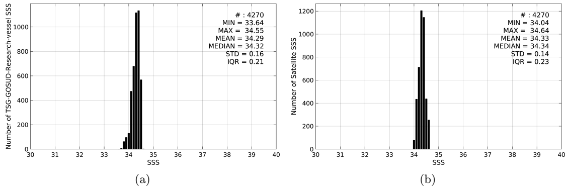
Figure 2: Histograms of SSS from TSG-GOSUD-Research-vessel (a) and SMAP-L3-JPL-V4-8DAY-RUNNING-60KM (b) considering all match-up pairs per bins of 0.1 over the North Pacific Ocean Pi-MEP region and for the full satellite product period.
