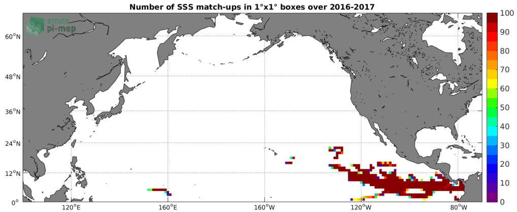
Figure 3: Number of SSS match-ups between Surface drifters SSS and the SMAP-L3-JPL-V4-8DAY-RUNNING-60KM SSS product for the North Pacific Ocean Pi-MEP region over 1°x1° boxes and for the full satellite product period.
