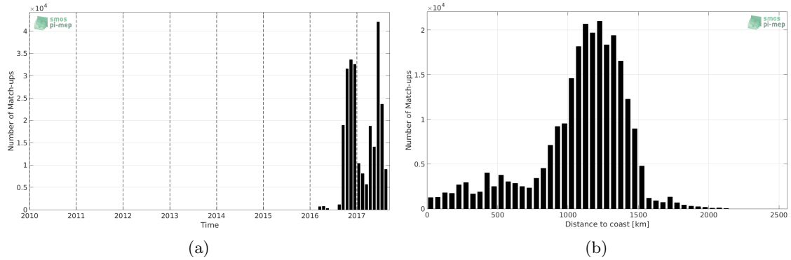
Figure 1: Number of match-ups between Surface drifters and SMAP-L3-JPL-V4-8DAY-RUNNING-60KM SSS as a function of time (a) and as function of the distance to coast (b) over the North Pacific Ocean Pi-MEP region and for the full satellite product period.
