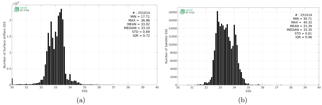
Figure 2: Histograms of SSS from Surface drifters (a) and SMAP-L3-JPL-V4-8DAY-RUNNING-60KM (b) considering all match-up pairs per bins of 0.1 over the North Pacific Ocean Pi-MEP region and for the full satellite product period.
