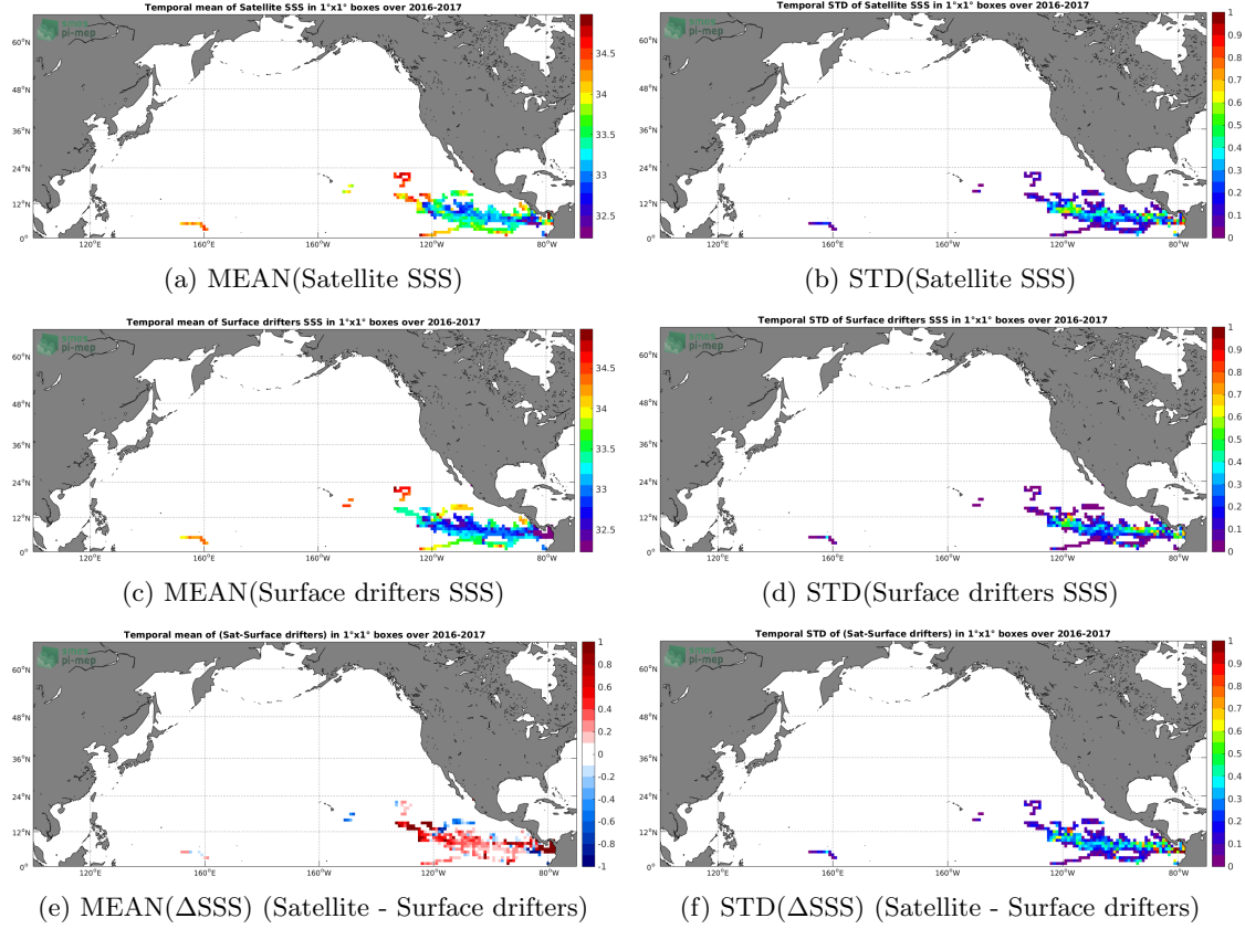
Figure 5: Temporal mean (left) and STD (right) of SSS from SMAP-L3-JPL-V4-8DAY-RUNNING-60KM (top), Surface drifters (middle), and of \Delta SSS (Satellite - Surface drifters). Only match-up pairs are used to generate these maps.
