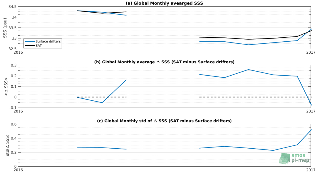
Figure 6: Time series of the monthly averaged mean SSS (top), mean \Delta \text{SSS} (Satellite - Surface drifters) and STD of \Delta \text{SSS} (Satellite - Surface drifters) over the North Pacific Ocean Pi-MEP region considering all match-ups collected by the Pi-MEP platform.
