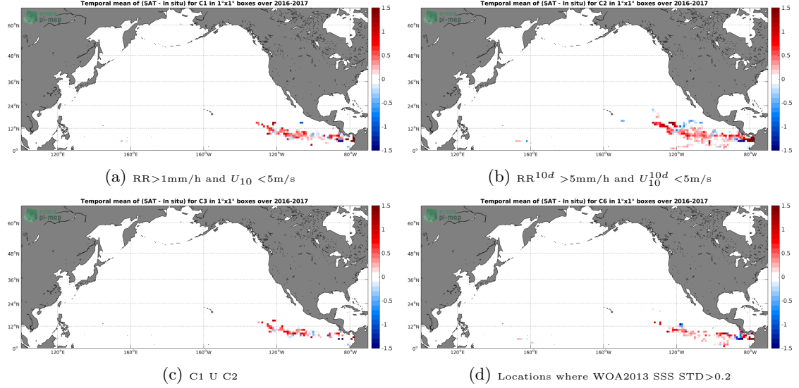
Figure 11: Temporal mean gridded over spatial boxes of size 1^\circ \times 1^\circ of \Delta SSS (SMAP-L3-JPL-V4-8DAY-RUNNING-60KM - Surface drifters) for 4 different subdatasets corresponding to: RR > 1\text{mm/h} and U_{10} < 5\text{m/s} (a), RR^{10d} > 5\text{mm/h} and U_{10}^{10d} < 5\text{m/s} (b), C1 U C2 (c), Locations where WOA2013 SSS STD > 0.2 (d).
